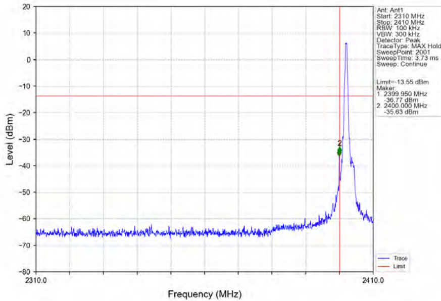
GFSK_DH5_LCH_2402MHz_Ant1_NTNV
