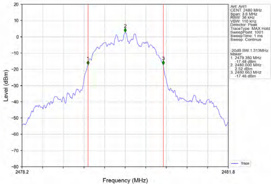
8DPSK_3DH5_HCH_2480MHz_Ant1_NTNV
