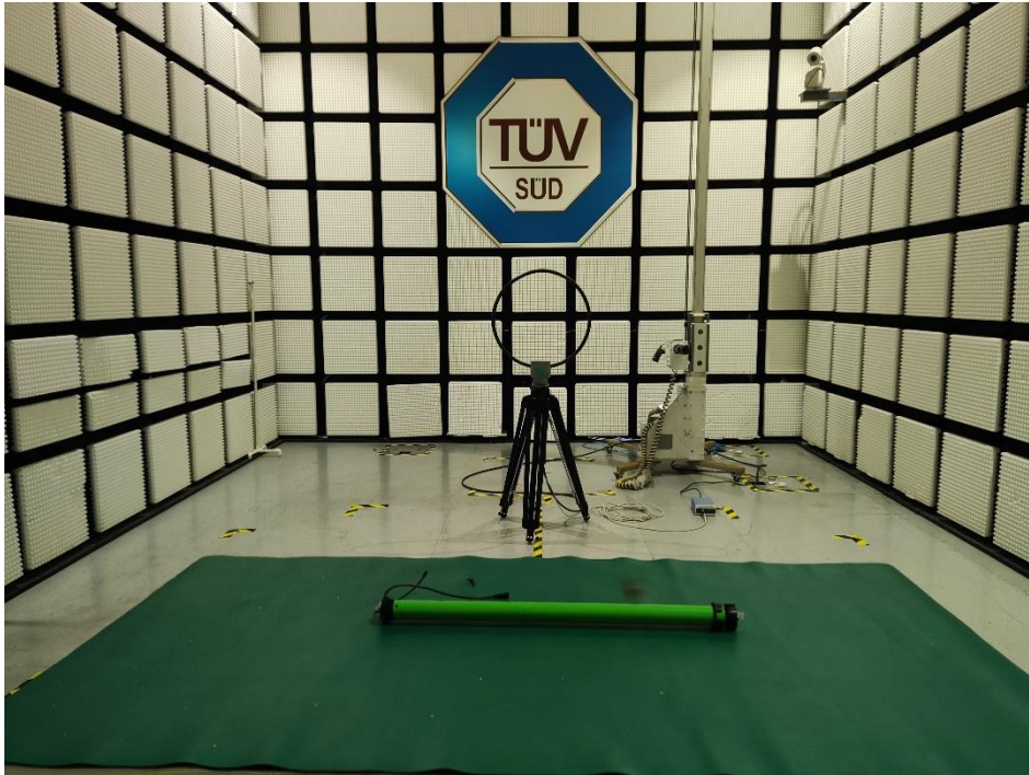
Radiated Emission Setup 9kHz ~ 30MHz DC mode
