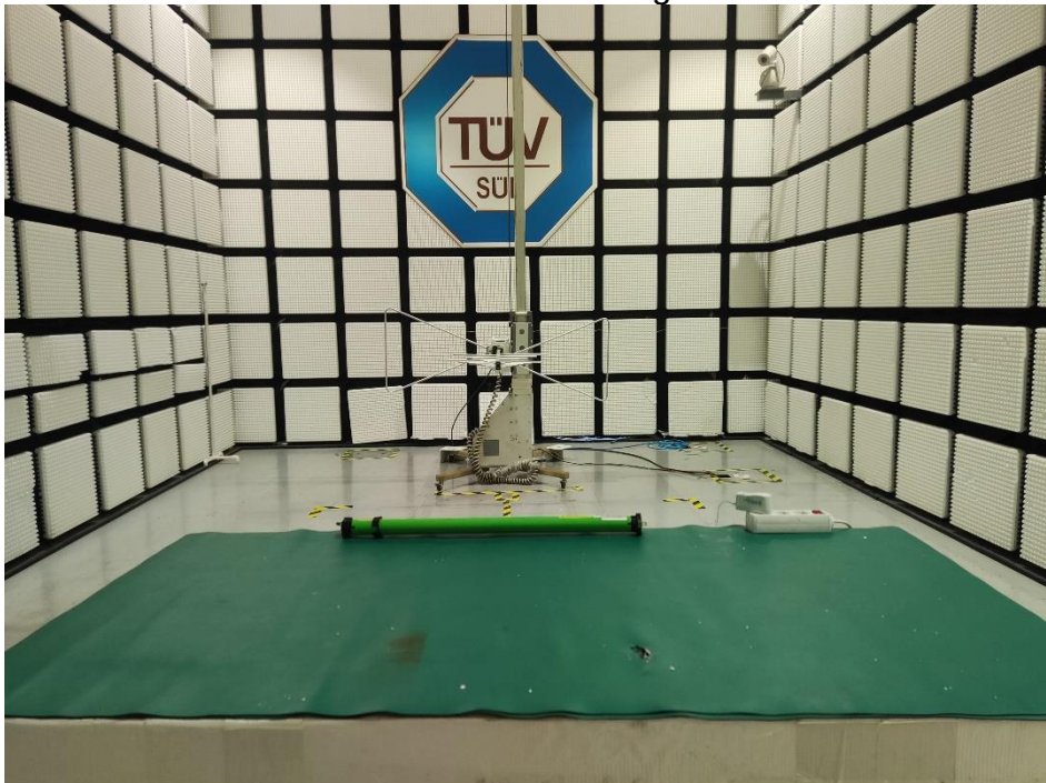
30MHz ~ 1GHz AC charge mode
