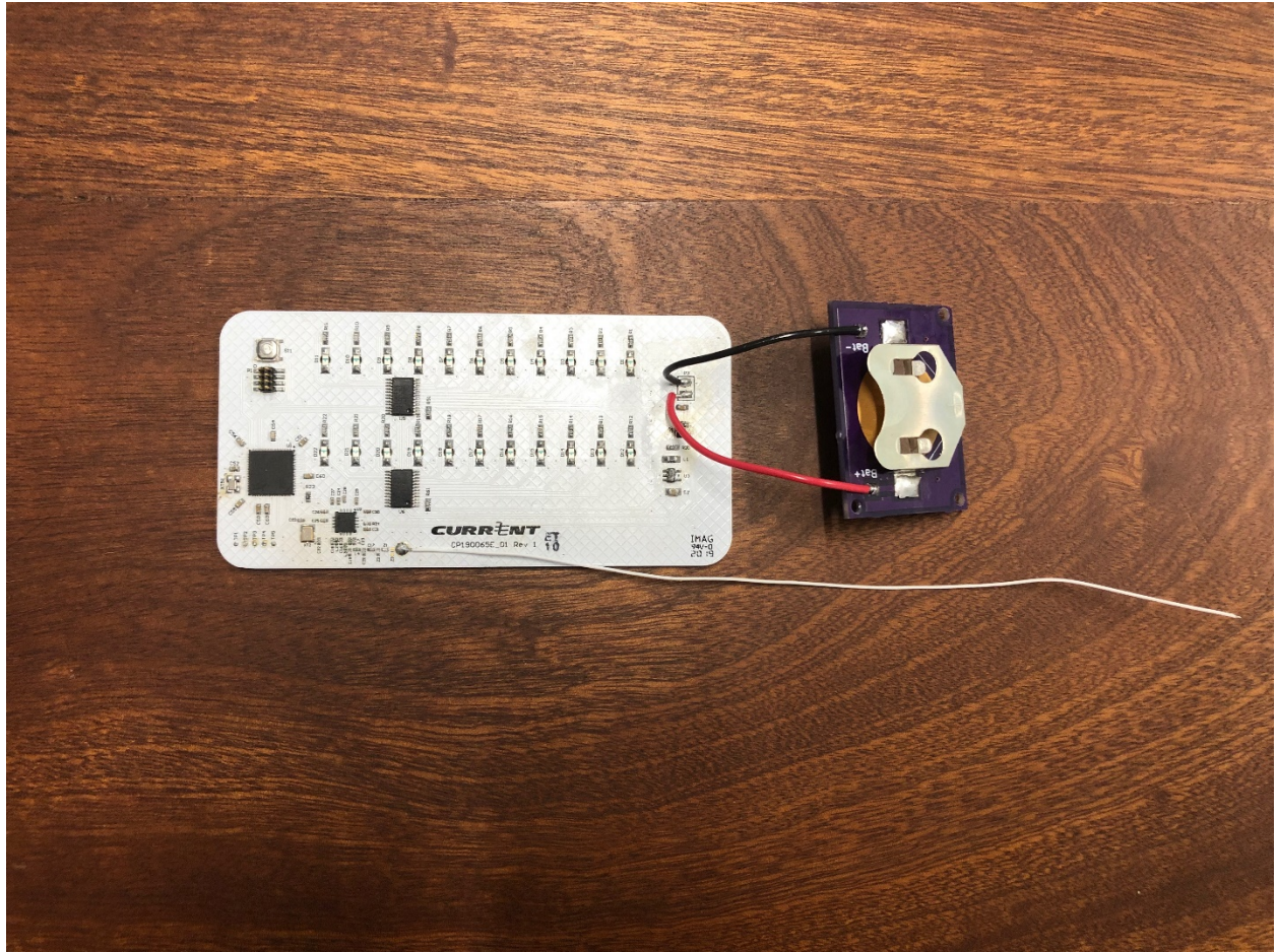
Figure 1: PCB View 1
