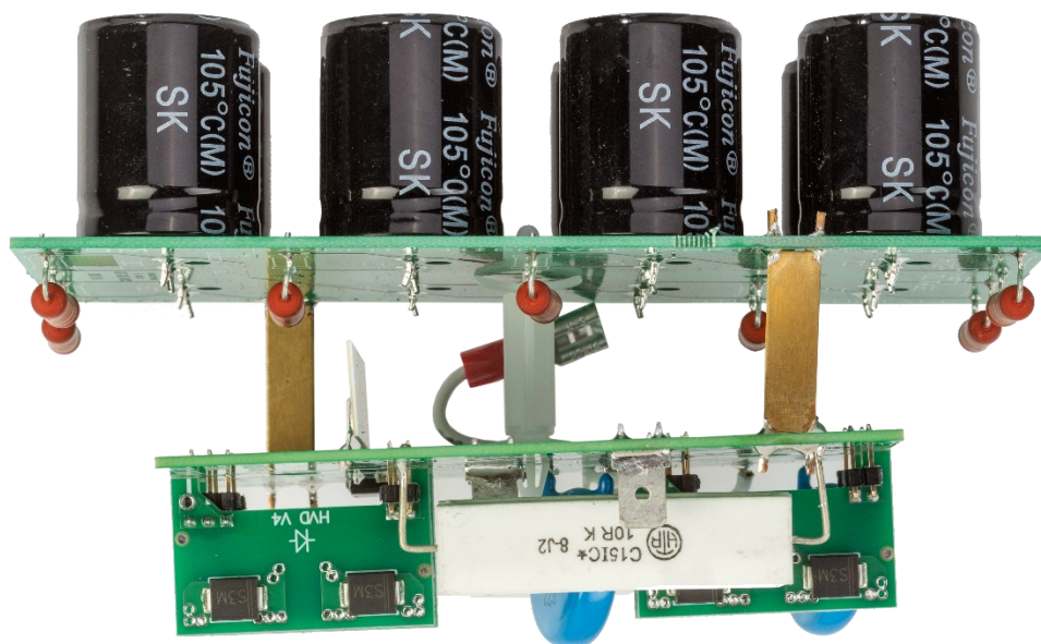
Figure 16 – HIGH VOLTAGE MODULE side view
