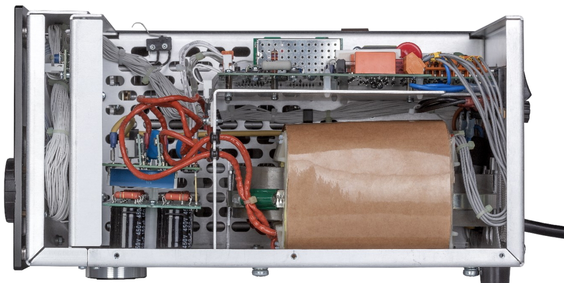
Figure 3 - ACOM 1003 left side view
