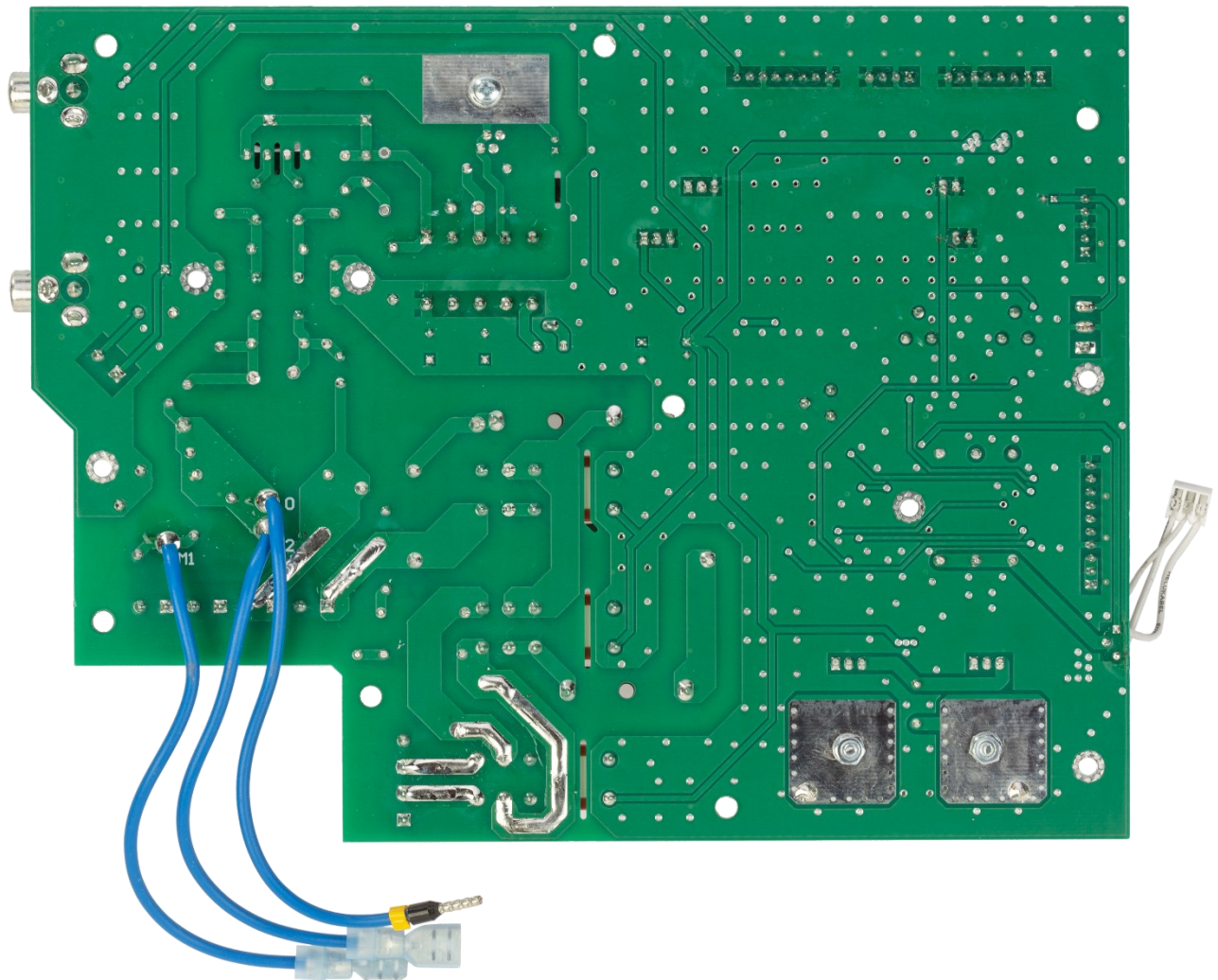
Figure 13 - A1003 Mains Board V2 bottom side
