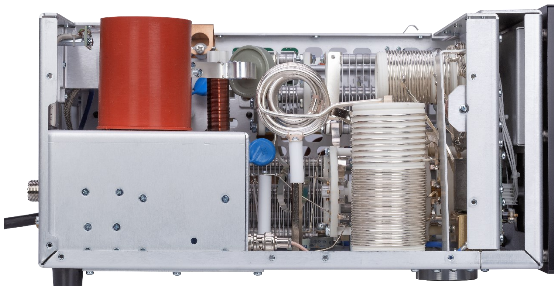
Figure 2 - ACOM 1003 right side view
