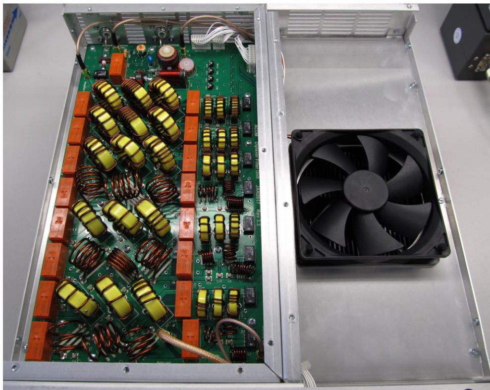
Fig.5 Bottom View
