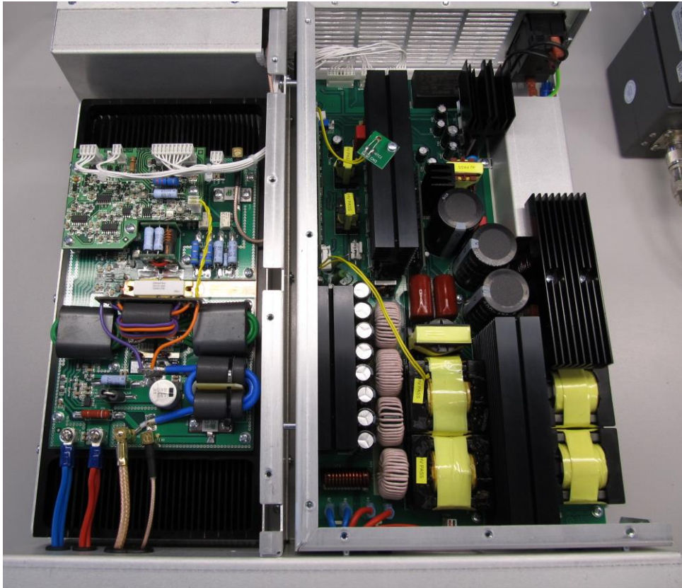
Fig.3 Top View
