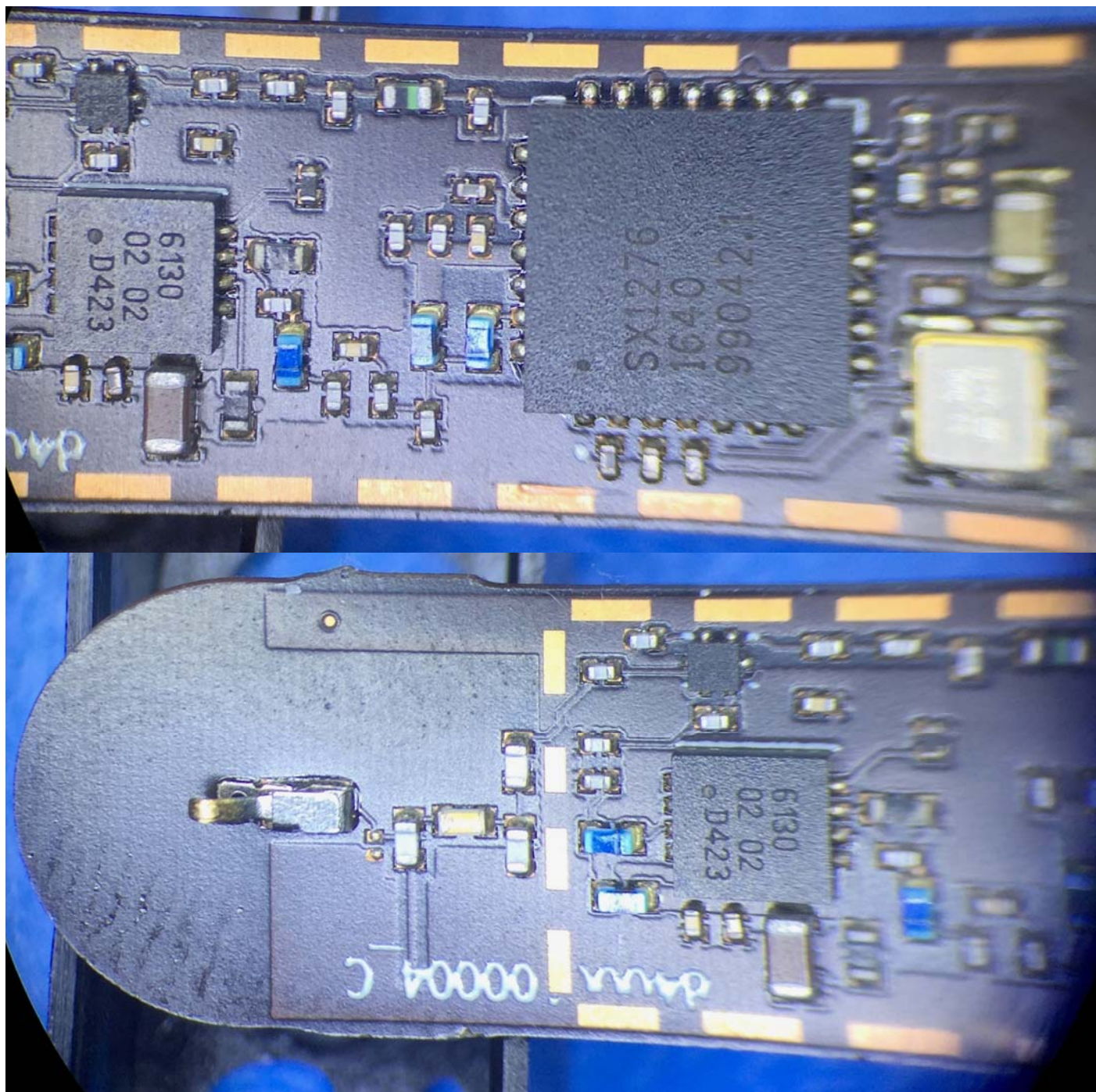
Figure 7 - Beartooth Radio BT 007 – LoRA chip & RF section
