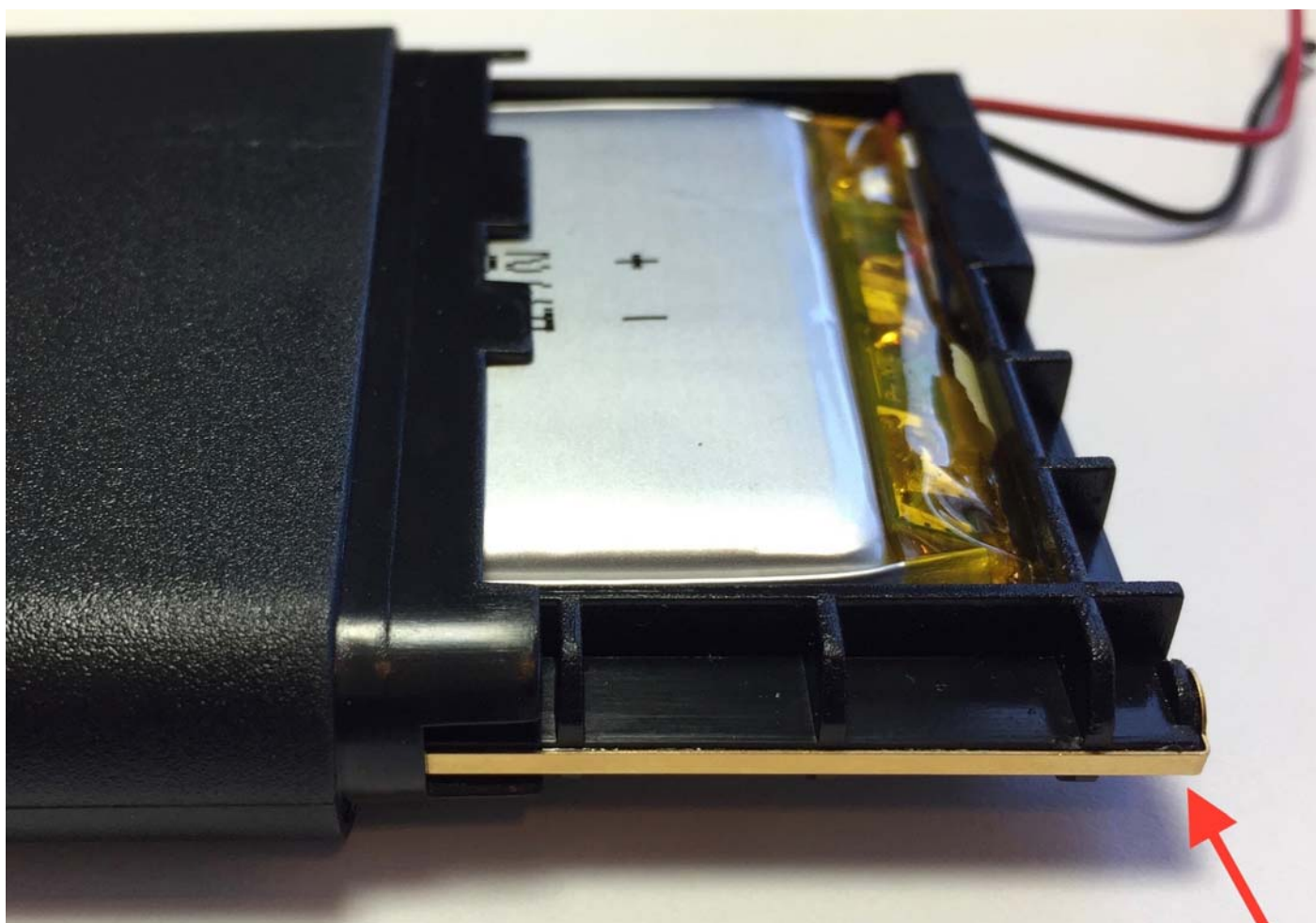
Figure 9 - Beartooth Radio BT 007 - LoRA antenna – angle 2
