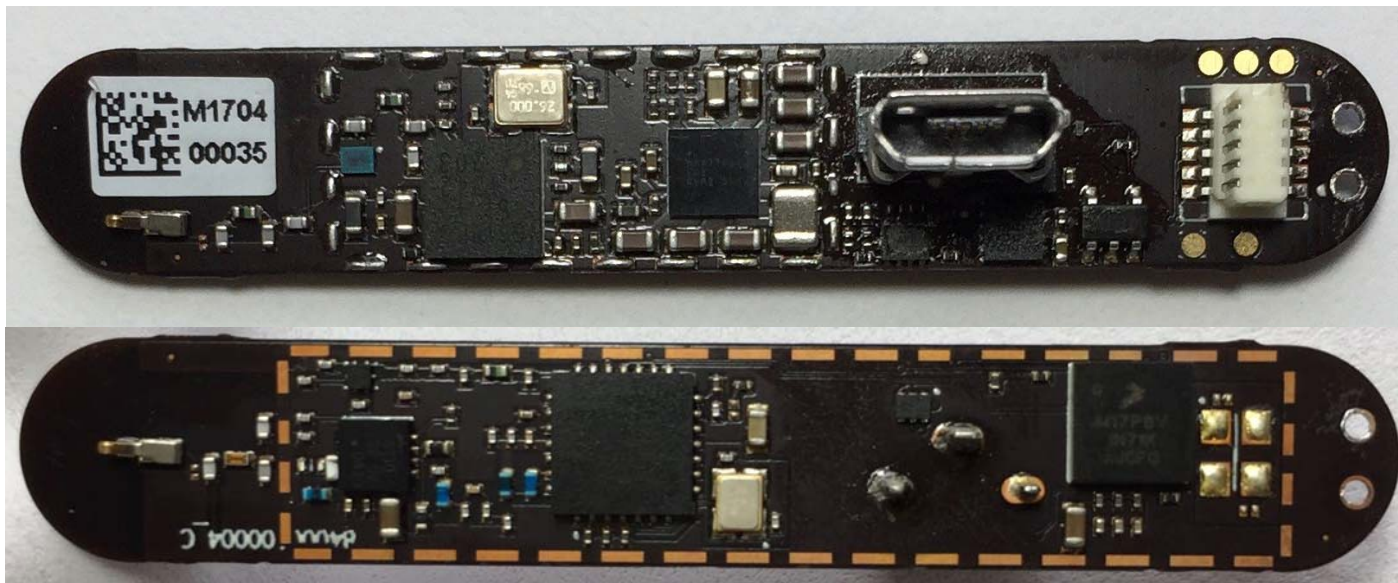
Figure 3 - Beartooth Radio BT 007 PWB 1 – front & back view
