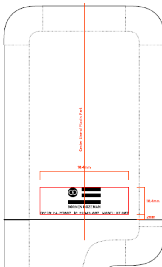
Figure 3 – Label Location, Scale 1:1
