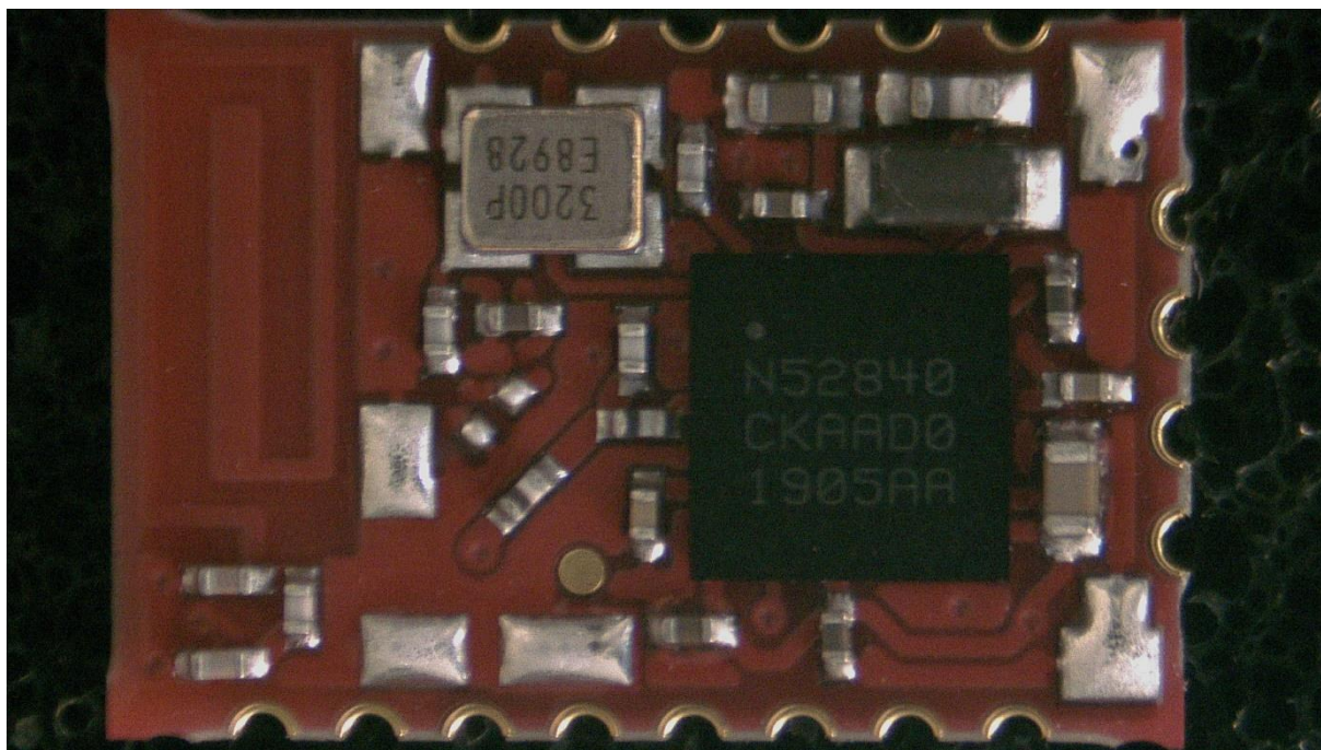
Figure 1 Top view
