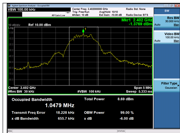
Ch 37 1M 99% OBW 1.05 MHz
