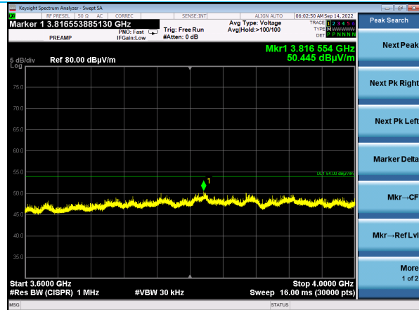
3600-4000 MHz Vertical Polarity EUT Horizontal Ch 37
