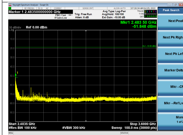
2483.5-3600 MHz Ch 39
