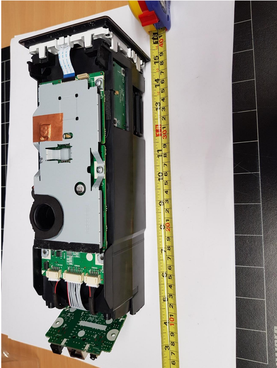
EUT Internal View 3
