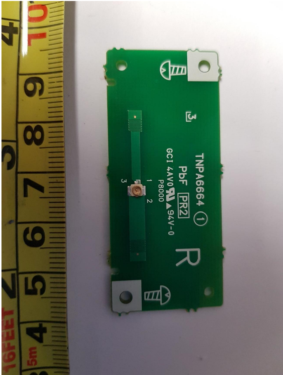
EUT Antenna PCB Component Side
