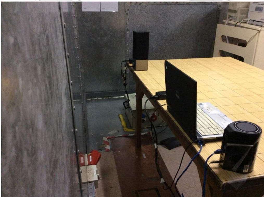
Conducted Emissions Test Setup (Rear View)
