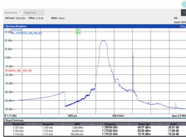
Band4-1.4MHz-QPSK-19957-6RB#0
