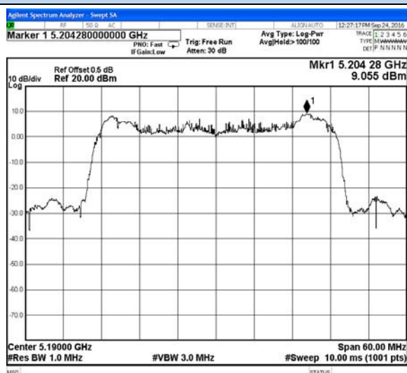
Chain 0-5190MHz
