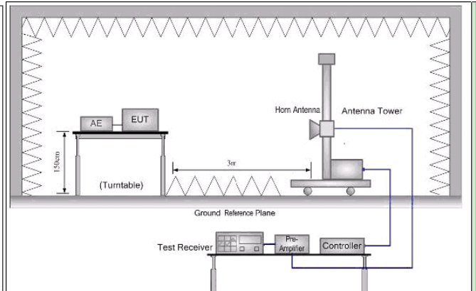
Figure 2. Above 1 GHz
