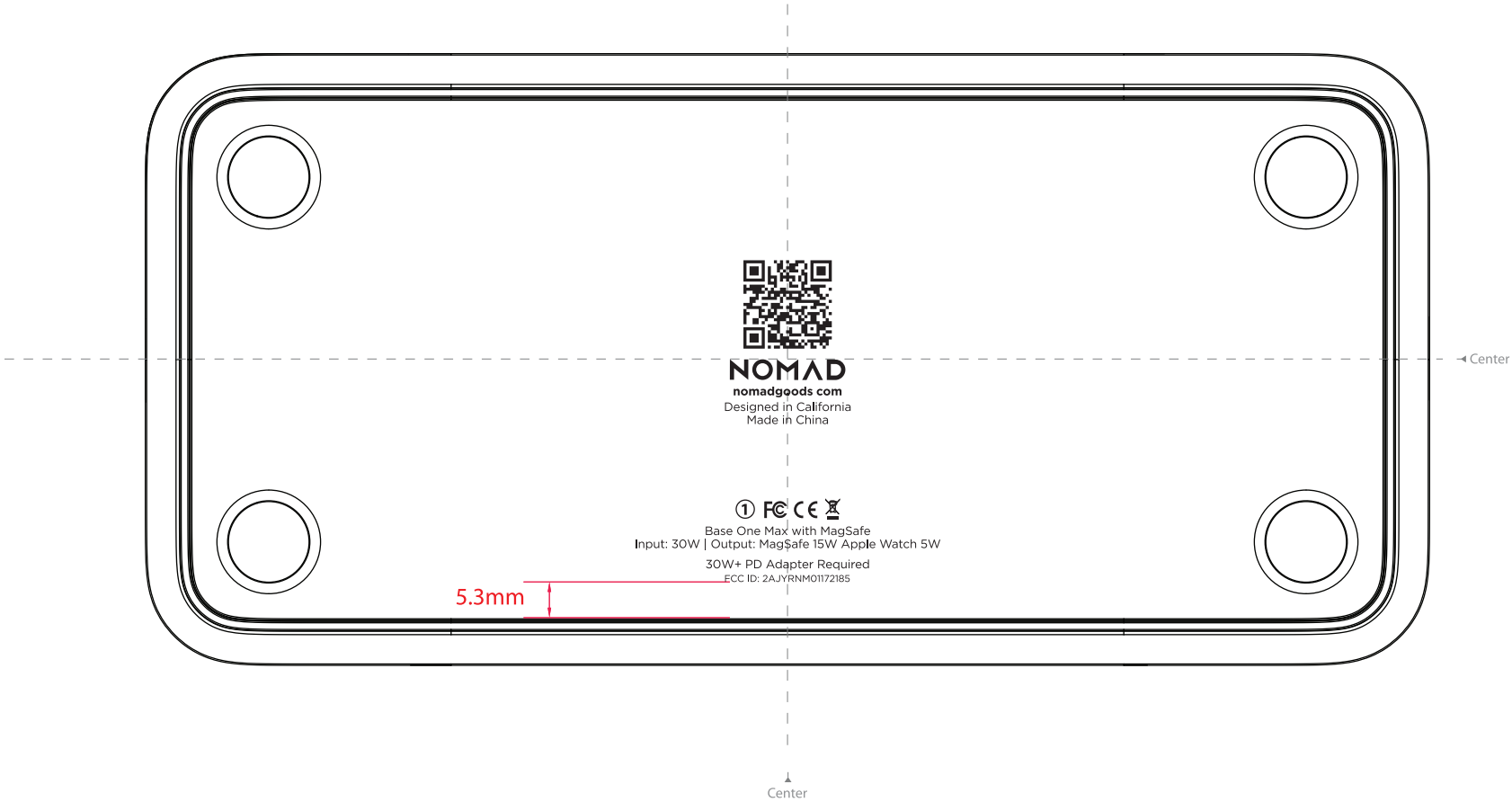
BOTTOM VIEW SCALE 1:1
