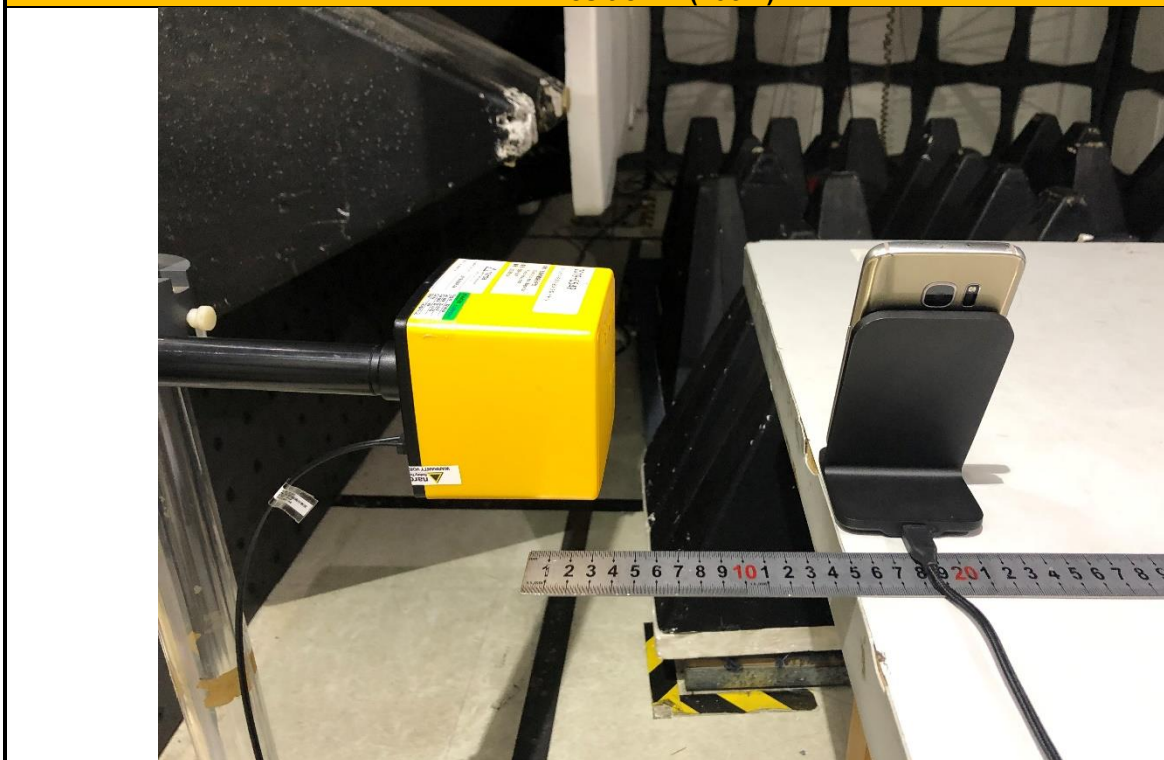
E-Field Strength and H-Field Strength Position B (15cm)
