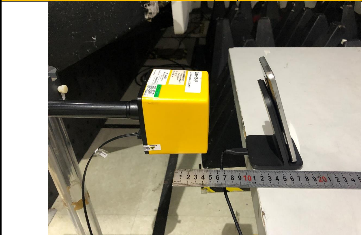
E-Field Strength and H-Field Strength Position D (15cm)
