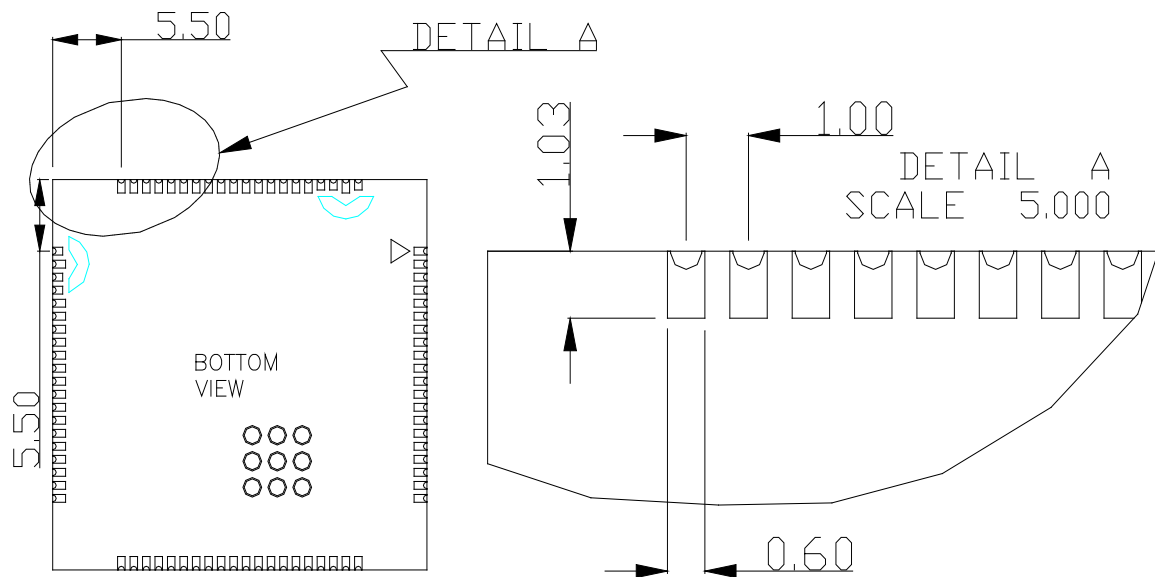
Figure 2: Dimention
