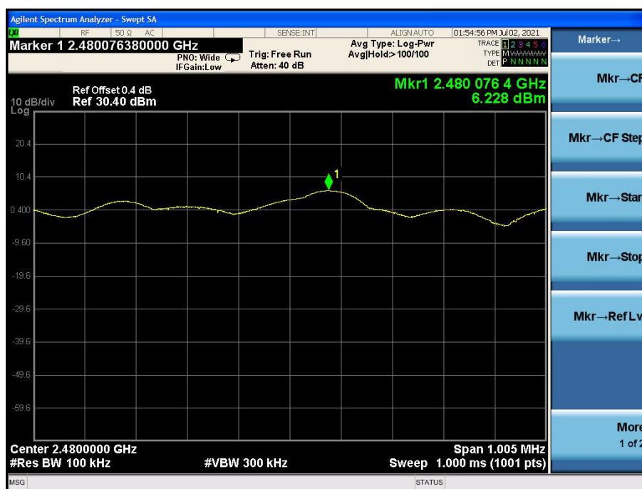
Fig.12 Power spectral density: 2M CH39 PSD/100KHz
