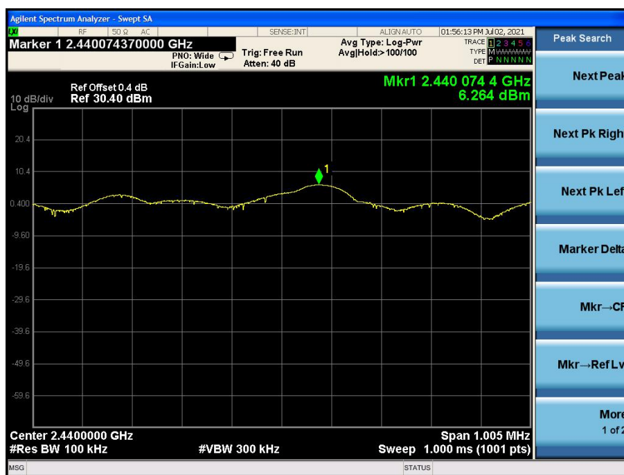
Fig.11 Power spectral density: 2M CH19 PSD/100KHz
