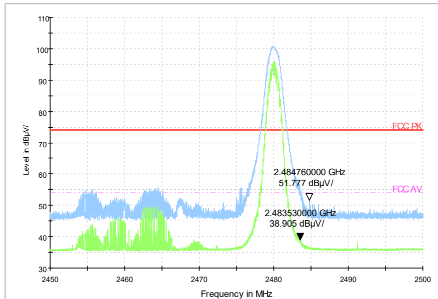
BAND EDGERE 1GHz-3GHz 2.45-2.5G
