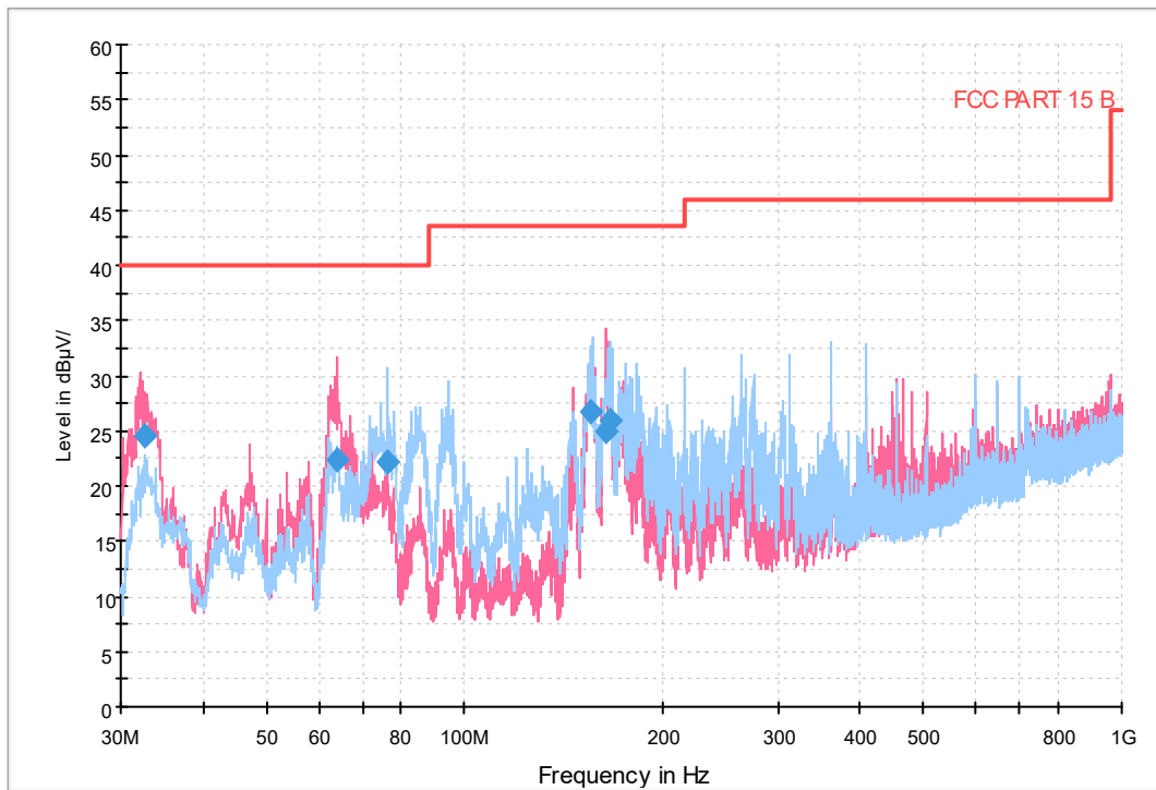
Fig.39 Radiated emission: Ch0, 30MHz-1GHz
