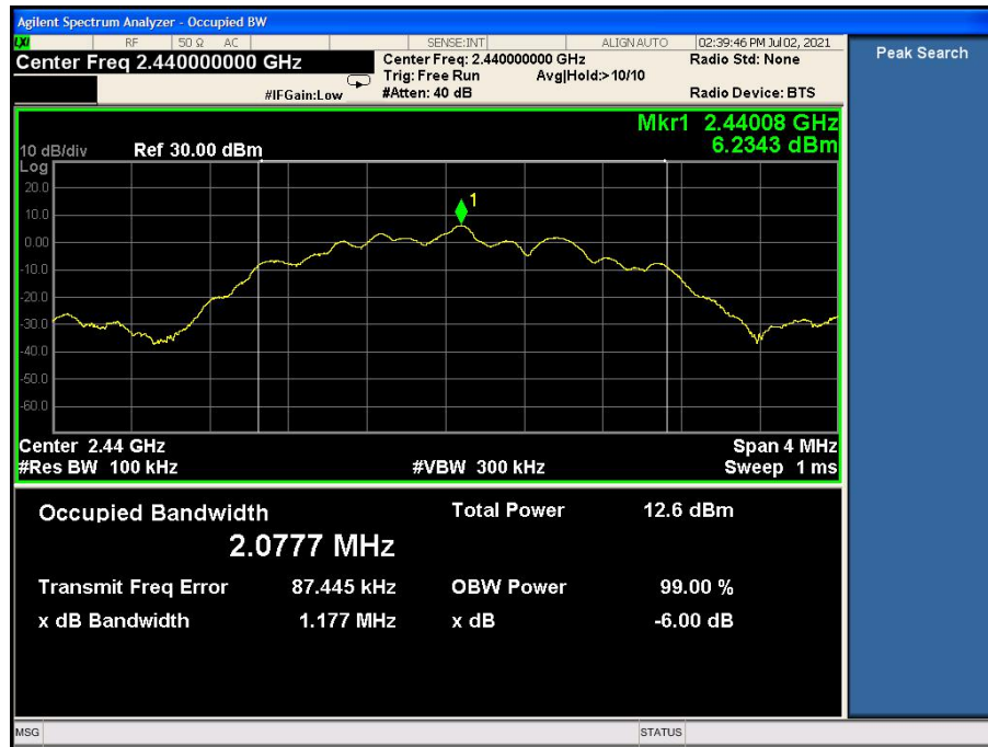
Fig.17 6dB Bandwidth: 2M Ch19
