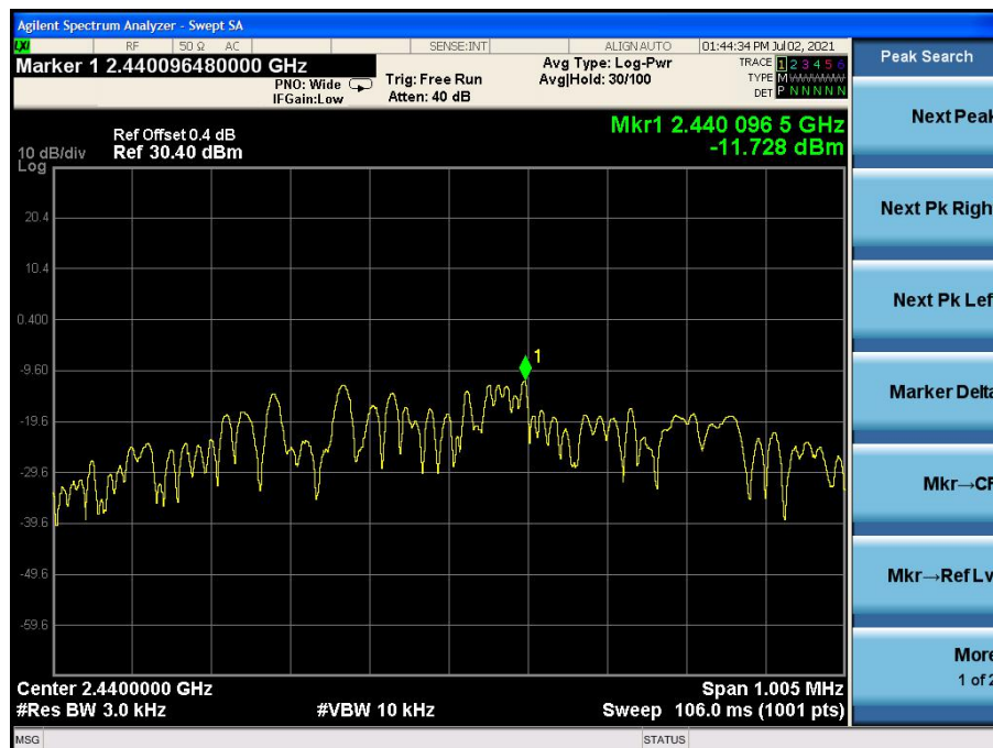
Fig.2 Power spectral density: 1M CH19 PSD/3KHz
