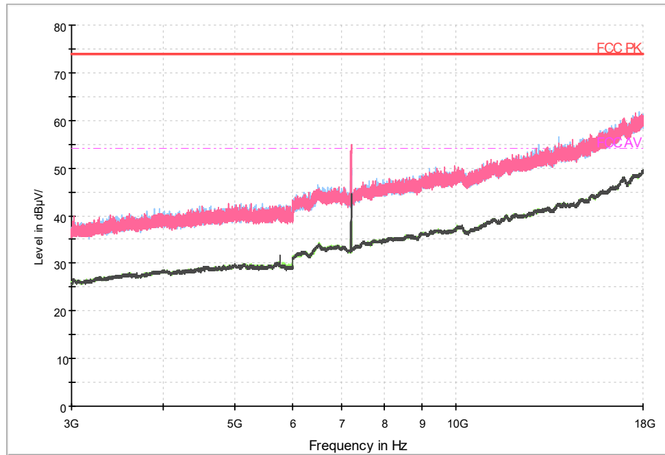
Fig.41 Radiated emission: Ch0, 3GHz-18GHz
