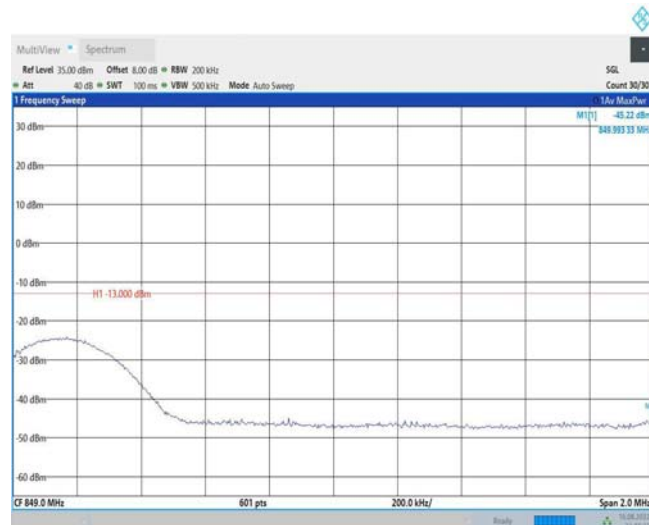
Band26-15MHz-16QAM-26965-1RB#74
