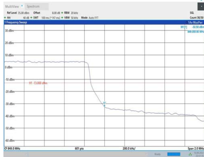
Band26-1.4MHz-16QAM-26697-1RB#0
