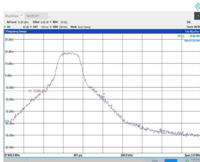
Band26-5MHz-16QAM-27015-25RB#0
