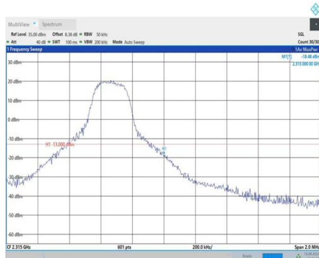
Band40-5MHz-QPSK-38775-25RB#0
