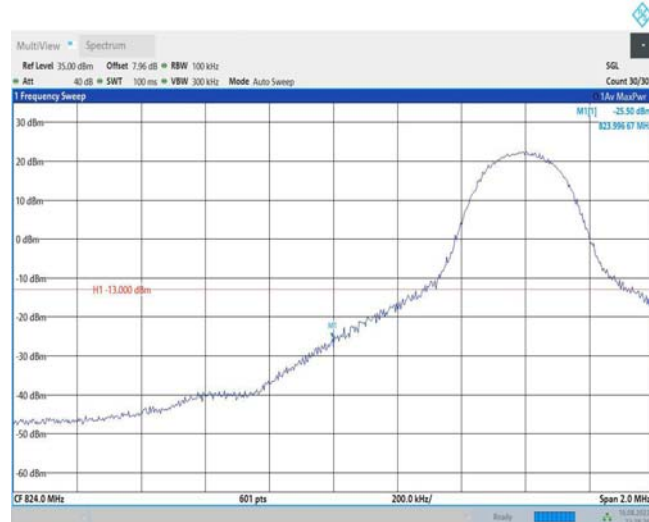
Band26-10MHz-QPSK-26840-1RB#49
