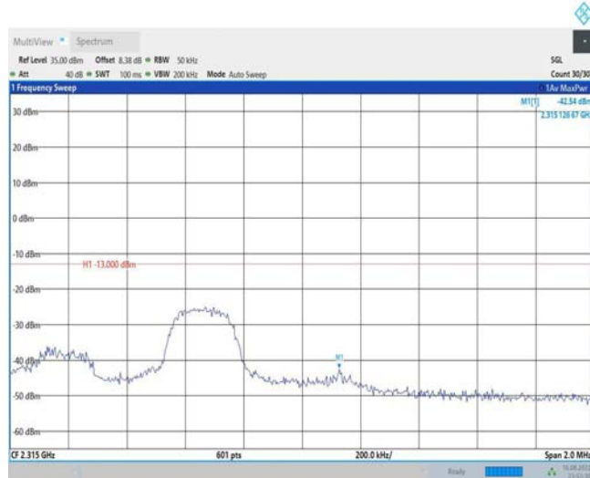
Band40-5MHz-16QAM-38775-1RB#24
