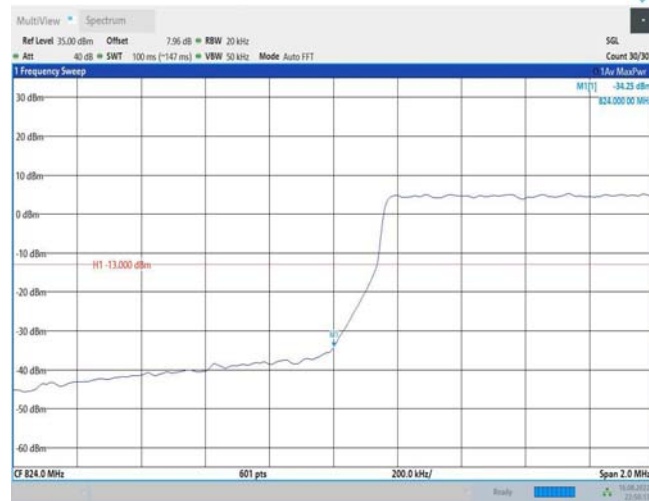
Band26-1.4MHz-16QAM-27033-1RB#0
