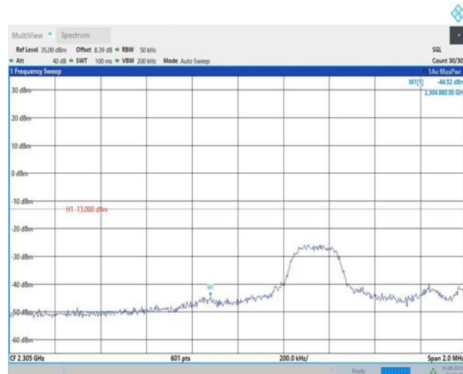
Band40-5MHz-16QAM-38725-25RB#0
