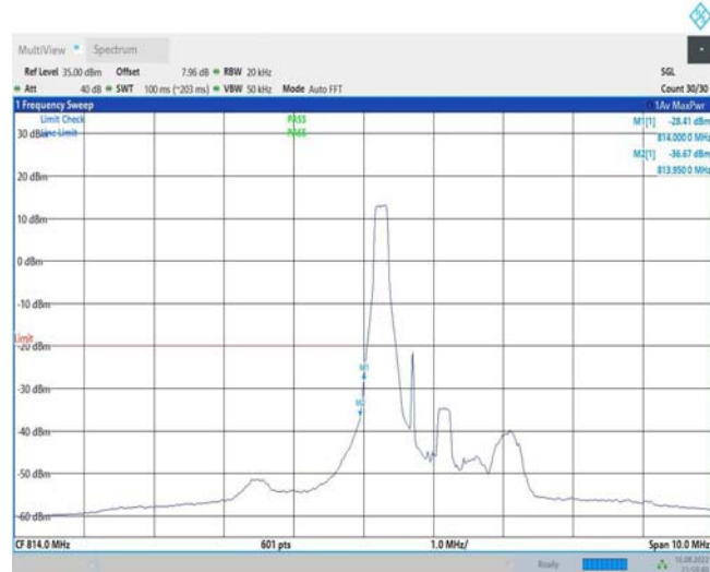
Band26-1.4MHz-16QAM-26697-1RB#5
