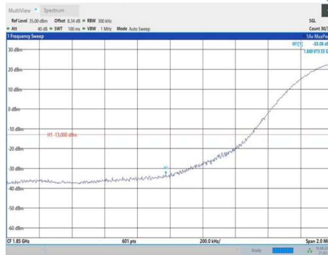
Band25-20MHz-16QAM-26140-1RB#99
