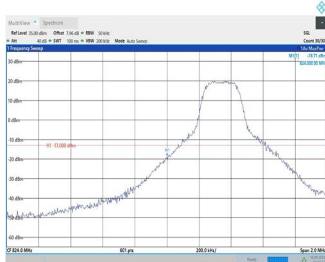
Band26-5MHz-QPSK-26815-1RB#24
