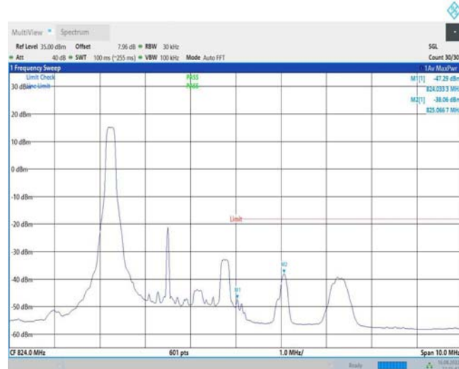
Band26-3MHz-QPSK-26775-1RB#14
