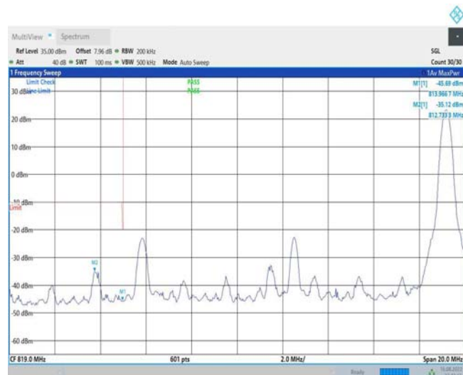
Band26-15MHz-QPSK-26765-75RB#0
