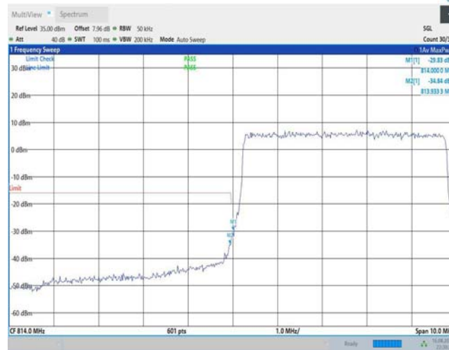
Band26-5MHz-QPSK-26765-1RB#0
