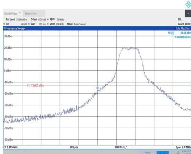
Band40-5MHz-QPSK-38725-1RB#24
