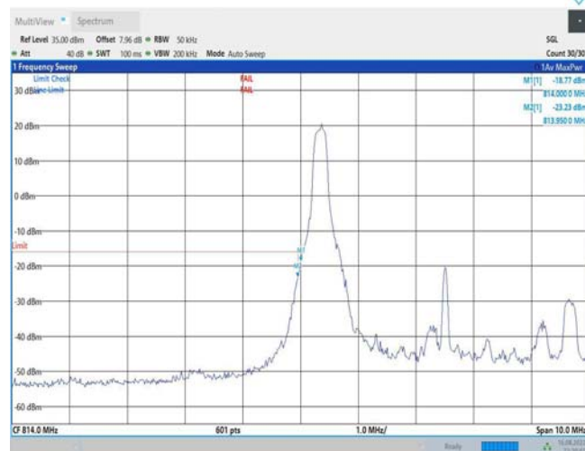
Band26-5MHz-16QAM-26715-1RB#24
