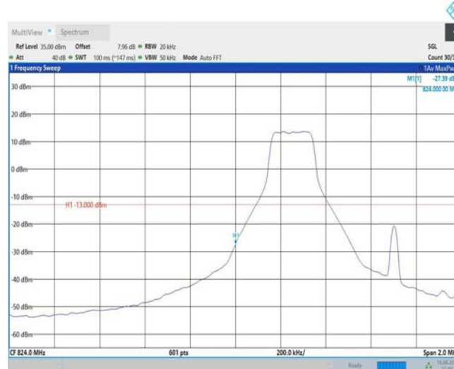
Band26-1.4MHz-16QAM-26797-1RB#5
