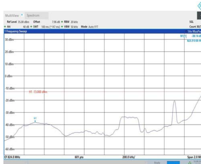
Band26-1.4MHz-16QAM-26797-6RB#0
