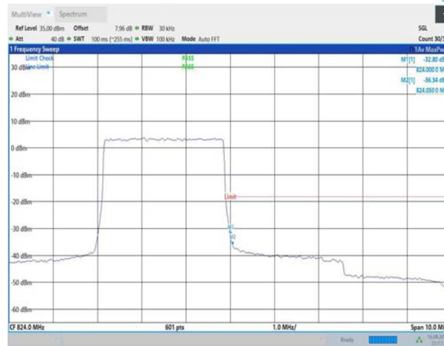
Band26-3MHz-QPSK-26805-1RB#0
