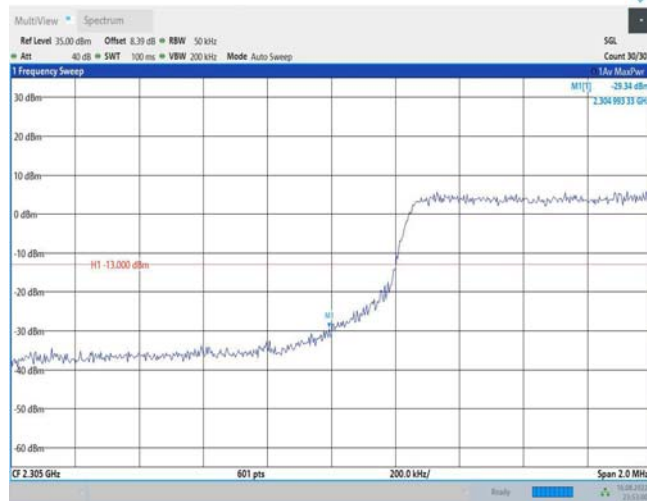
Band40-5MHz-16QAM-38775-1RB#0
