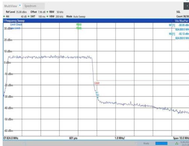
Band26-5MHz-16QAM-26815-1RB#0
