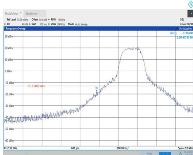
Band40-5MHz-16QAM-39175-1RB#24
