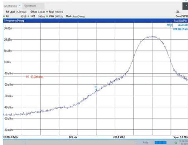
Band26-10MHz-16QAM-26840-1RB#49
