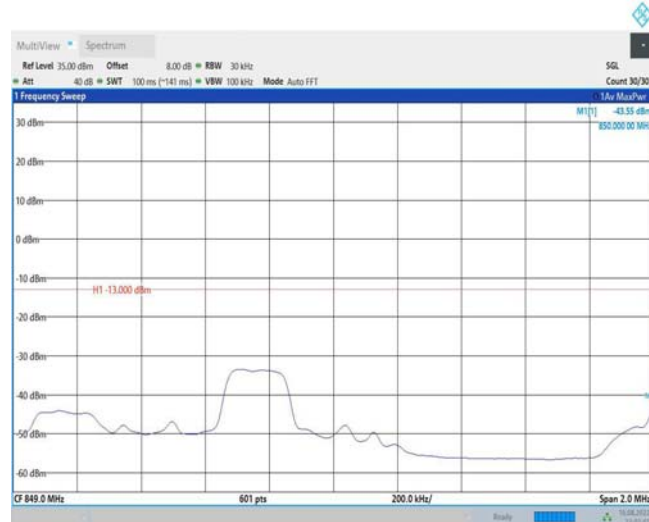
Band26-3MHz-16QAM-27025-1RB#14
