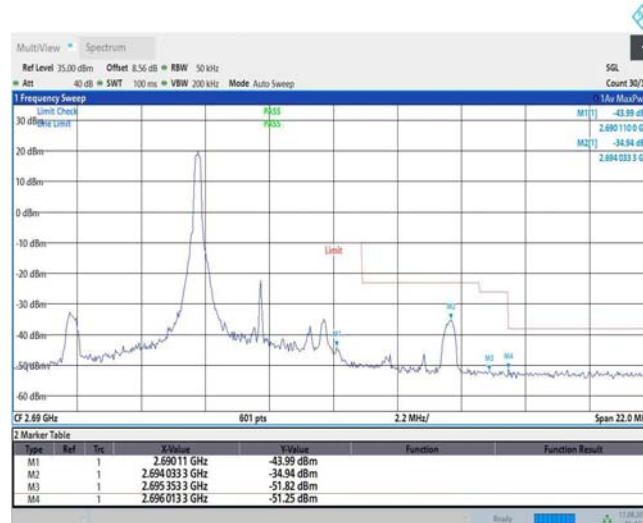
Band41-5MHz-QPSK-41565-1RB#24
