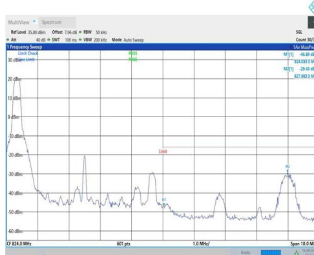
Band26-5MHz-16QAM-26765-1RB#24
