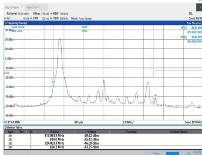
Band26-10MHz-QPSK-26740-1RB#49
