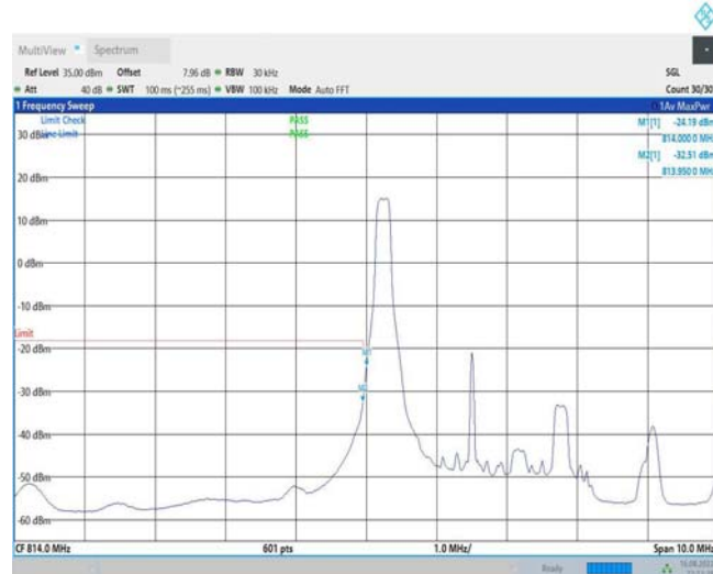
Band26-3MHz-16QAM-26705-1RB#14
