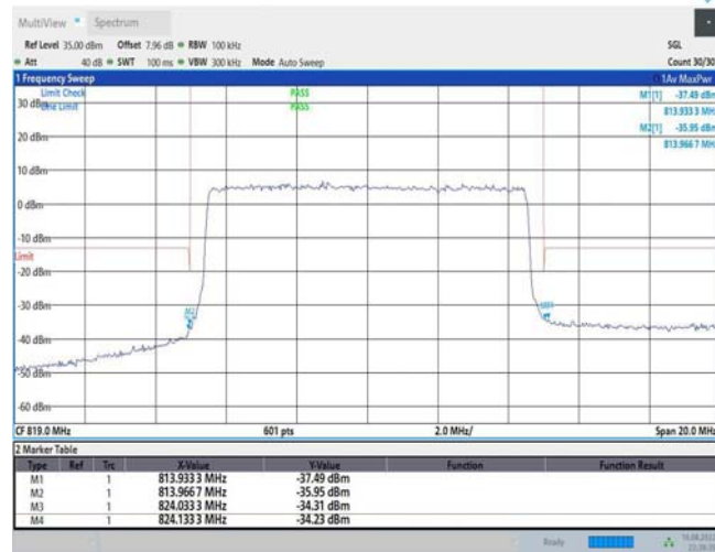
Band26-10MHz-QPSK-26840-1RB#0
