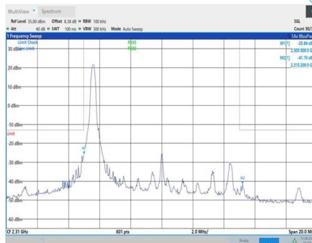
Band40-10MHz-16QAM-38750-1RB#49
