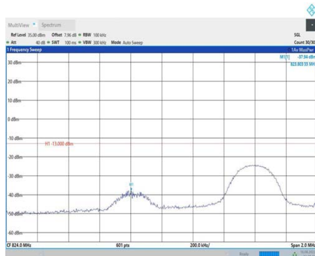
Band26-10MHz-QPSK-26840-50RB#0
