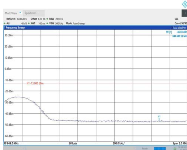
Band26-15MHz-QPSK-26965-1RB#74
