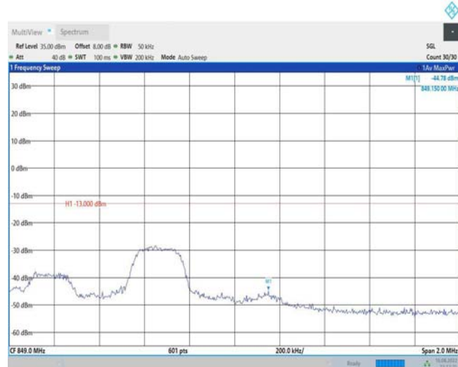
Band26-5MHz-QPSK-27015-1RB#24
