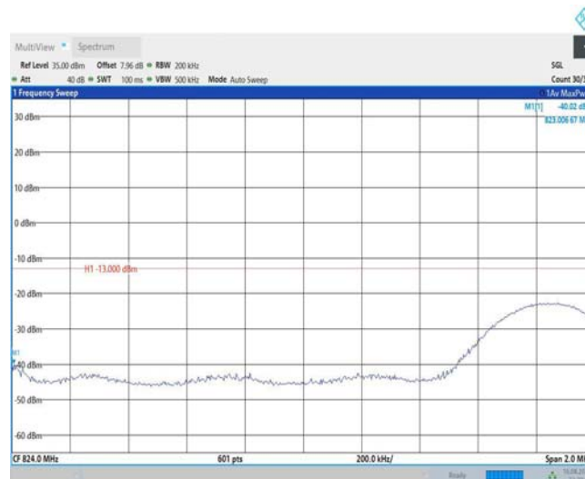
Band26-15MHz-QPSK-26865-75RB#0
