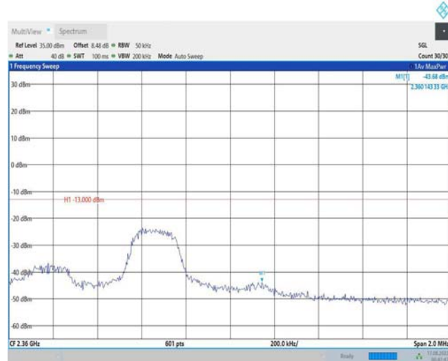
Band40-5MHz-16QAM-39225-1RB#24
