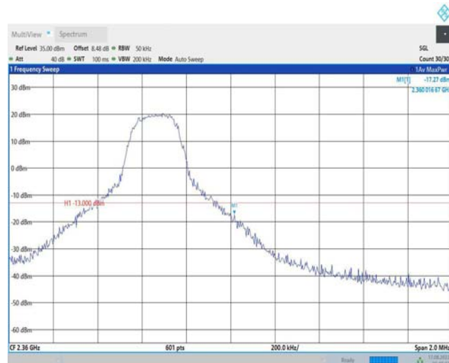
Band40-5MHz-16QAM-39225-25RB#0
