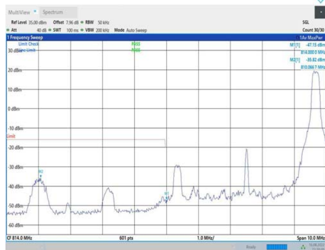
Band26-5MHz-QPSK-26715-25RB#0
