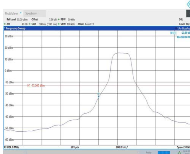
Band26-3MHz-QPSK-26805-1RB#14
