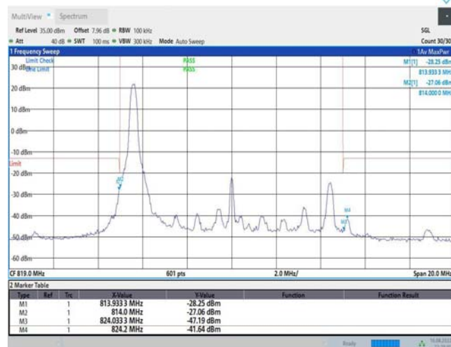
Band26-10MHz-16QAM-26740-1RB#49
