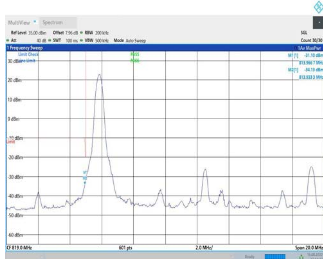
Band26-15MHz-QPSK-26765-1RB#74
