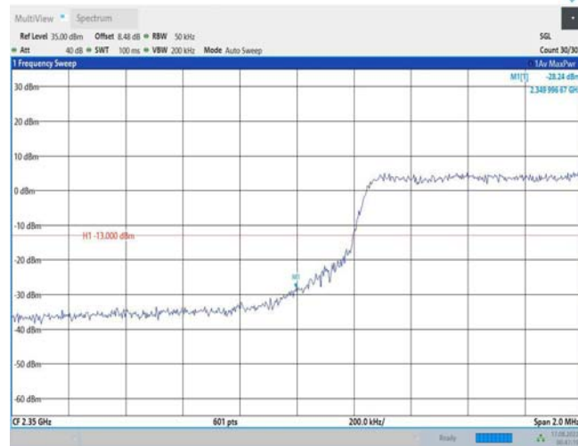
Band40-5MHz-16QAM-39225-1RB#0
