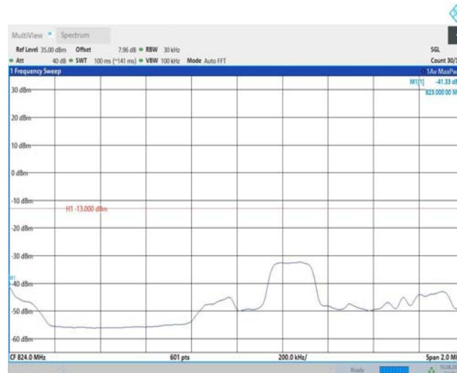
Band26-3MHz-QPSK-26805-15RB#0
