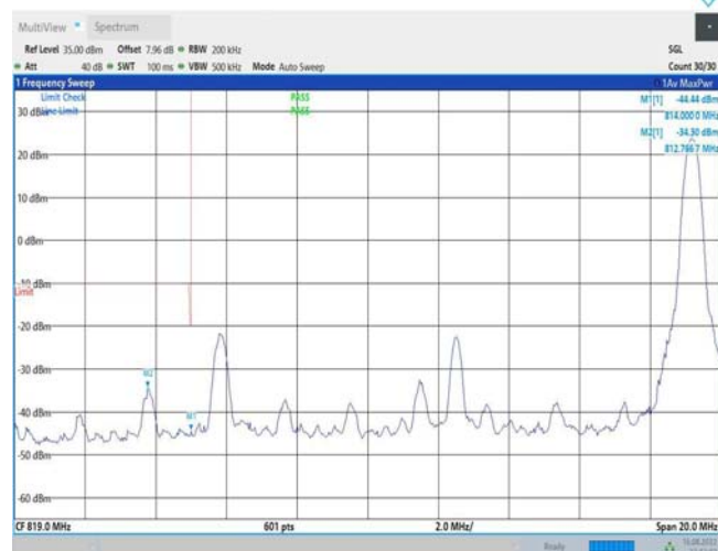
Band26-15MHz-16QAM-26865-1RB#0
