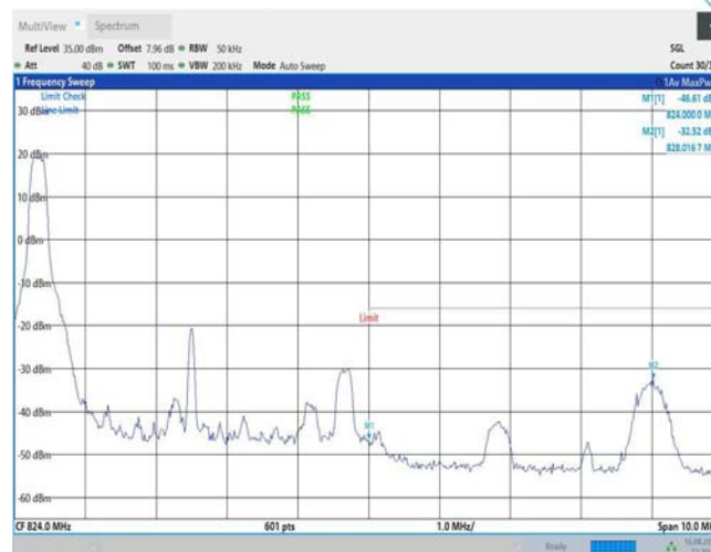
Band26-5MHz-QPSK-26765-1RB#24
