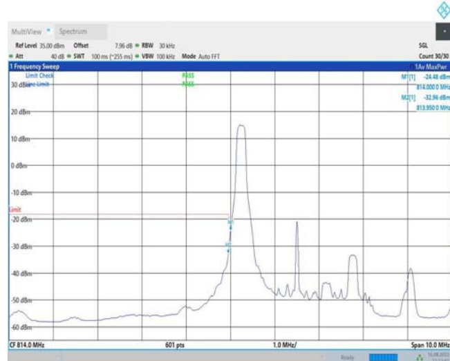
Band26-3MHz-QPSK-26705-1RB#14
