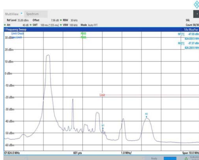
Band26-3MHz-16QAM-26775-1RB#14
