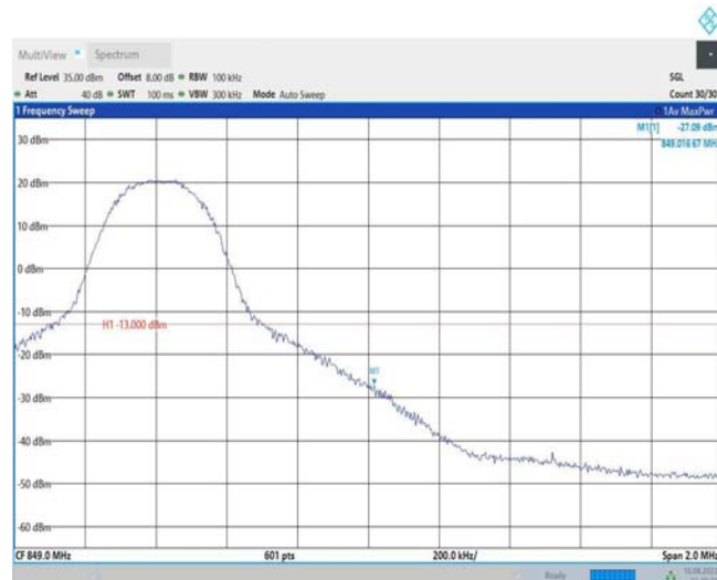
Band26-10MHz-QPSK-26990-50RB#0
