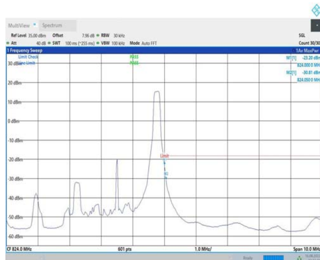
Band26-3MHz-16QAM-26775-15RB#0
