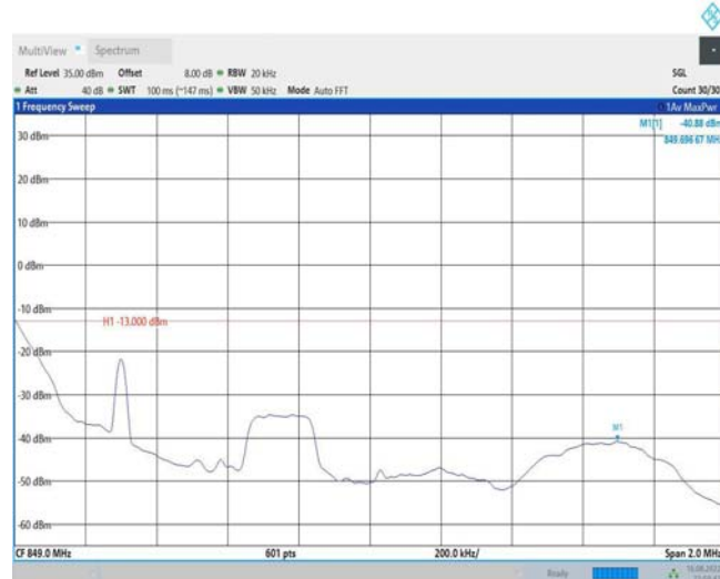
Band26-1.4MHz-QPSK-27033-1RB#5
