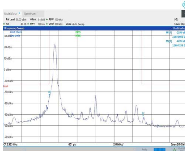
Band40-10MHz-QPSK-39200-1RB#49
