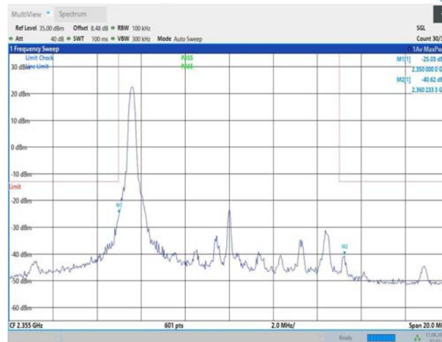
Band40-10MHz-16QAM-39200-1RB#49
