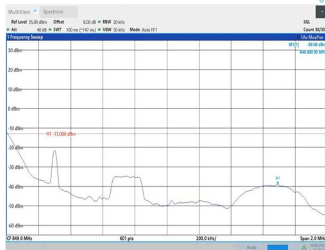
Band26-1.4MHz-16QAM-27033-1RB#5
