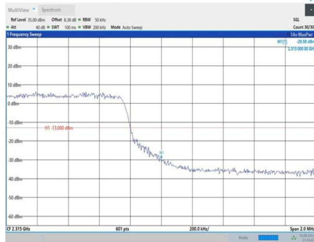
Band40-5MHz-16QAM-39175-1RB#0
