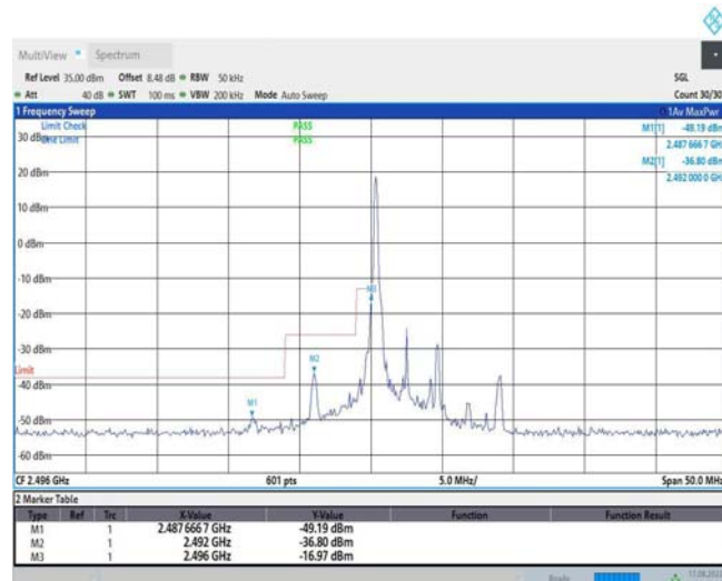
Band41-5MHz-16QAM-39675-1RB#24
