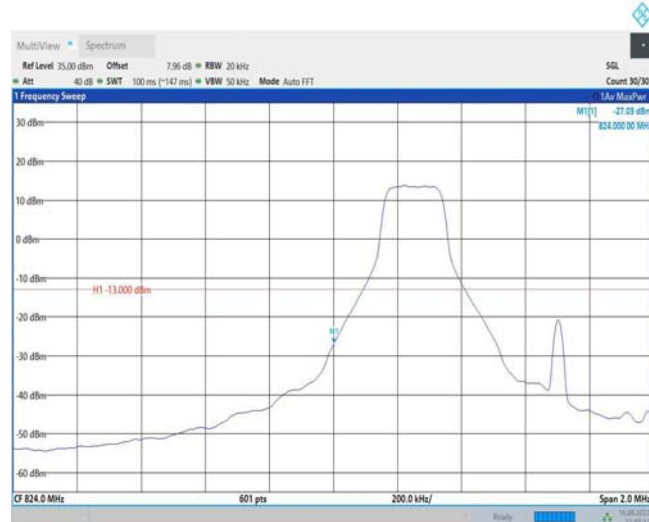
Band26-1.4MHz-QPSK-26797-1RB#5
