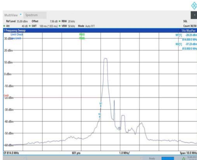
Band26-1.4MHz-QPSK-26697-1RB#5
