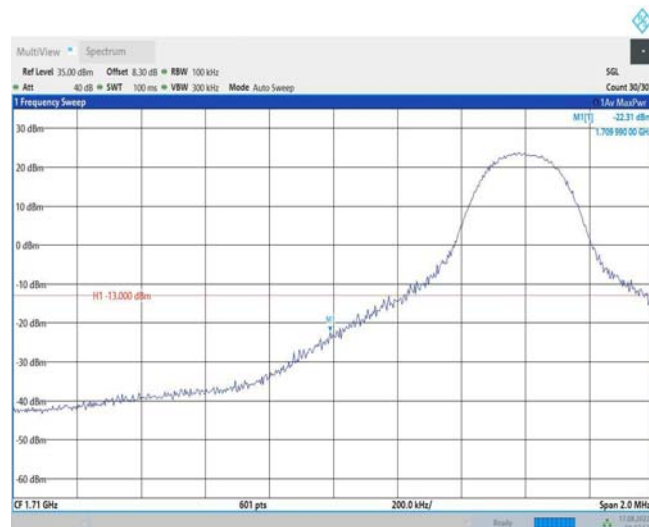
Band66-10MHz-QPSK-132022-1RB#49
