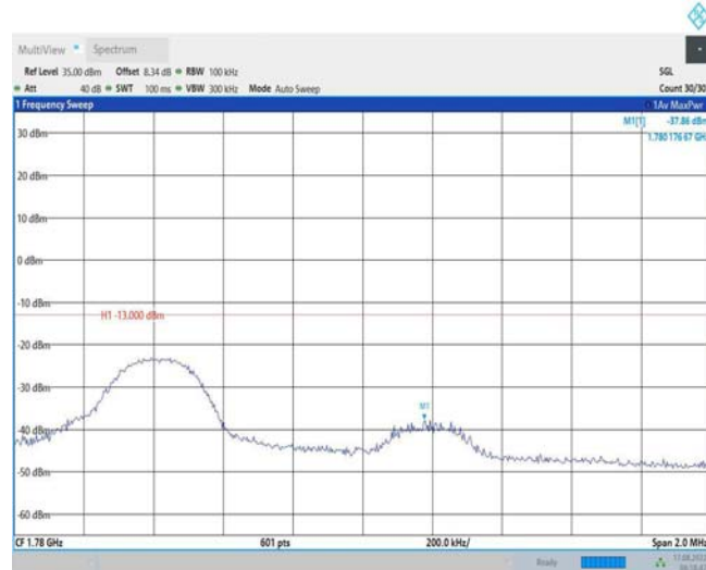
Band66-10MHz-16QAM-132622-1RB#49
