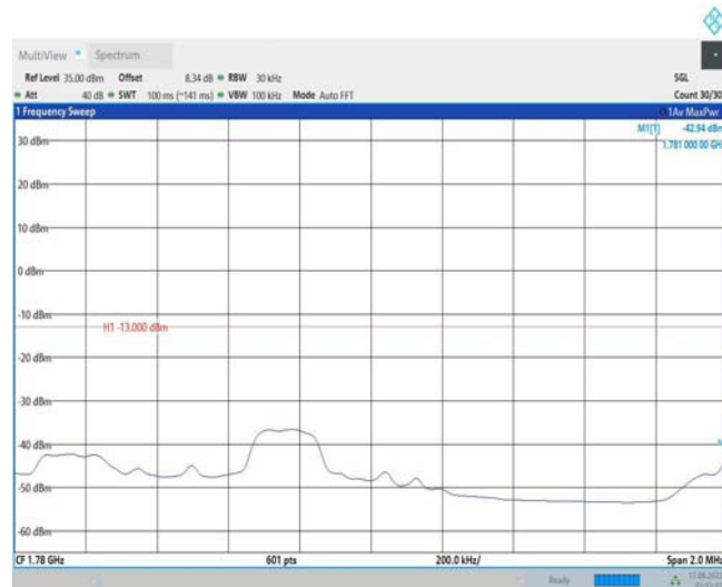
Band66-3MHz-QPSK-132657-1RB#14
