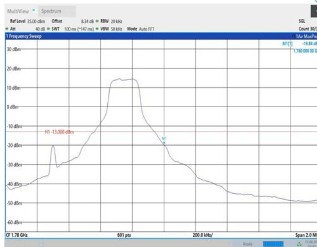
Band66-1.4MHz-QPSK-132665-6RB#0
