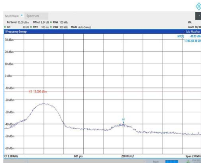
Band66-10MHz-QPSK-132622-1RB#49
