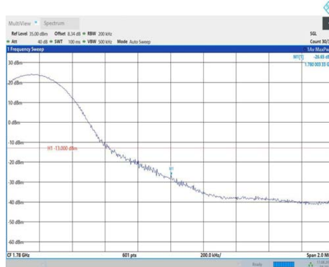
Band66-15MHz-QPSK-132597-75RB#0
