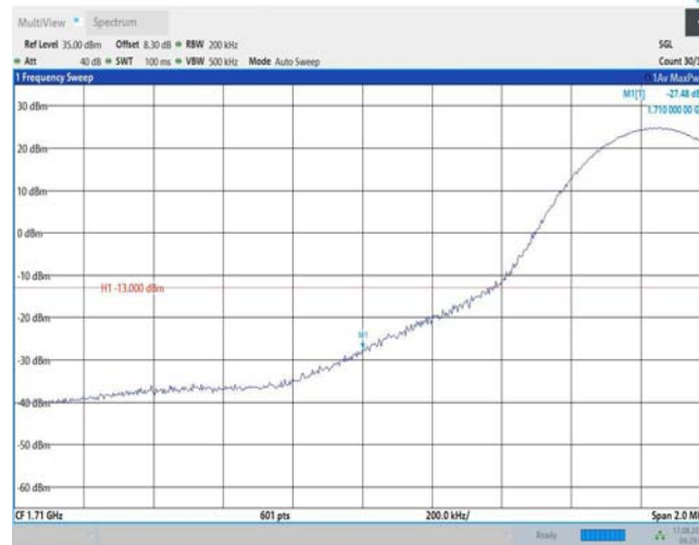
Band66-15MHz-QPSK-132047-1RB#74
