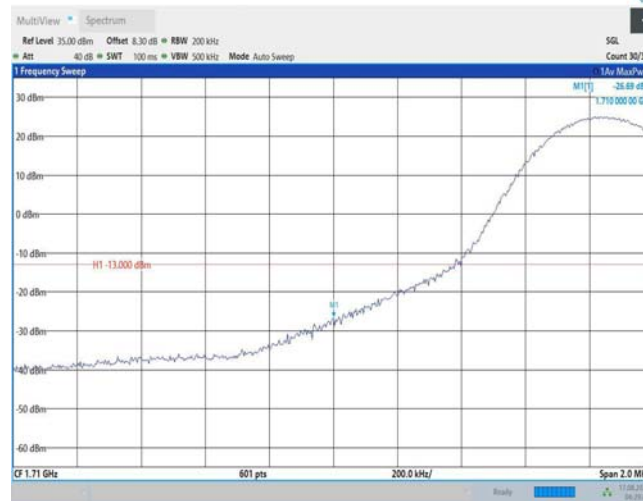
Band66-15MHz-16QAM-132047-1RB#74
