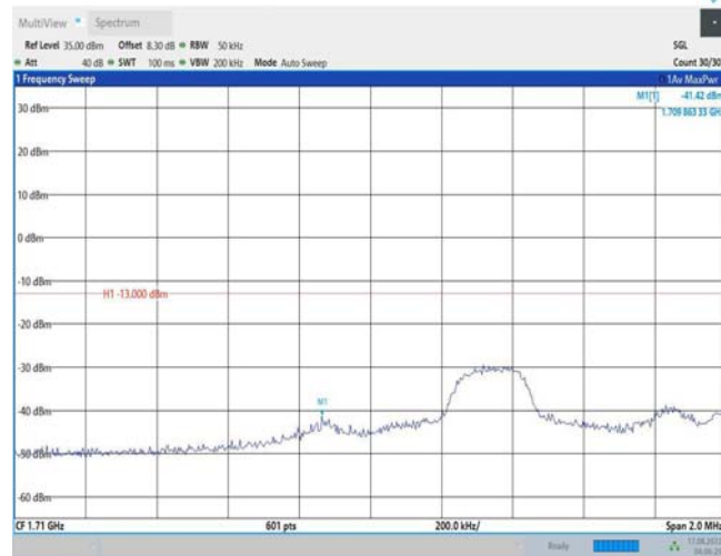
Band66-5MHz-QPSK-131997-25RB#0
