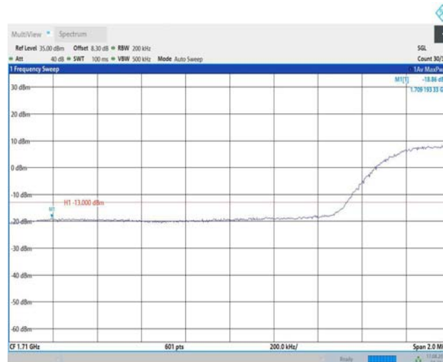
Band66-15MHz-QPSK-132597-1RB#0
