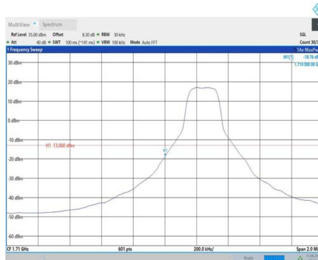
Band66-3MHz-QPSK-131987-1RB#14
