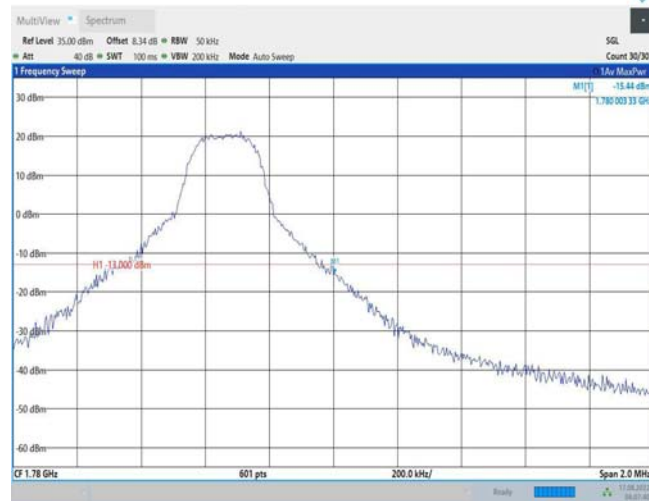
Band66-5MHz-16QAM-132647-25RB#0
