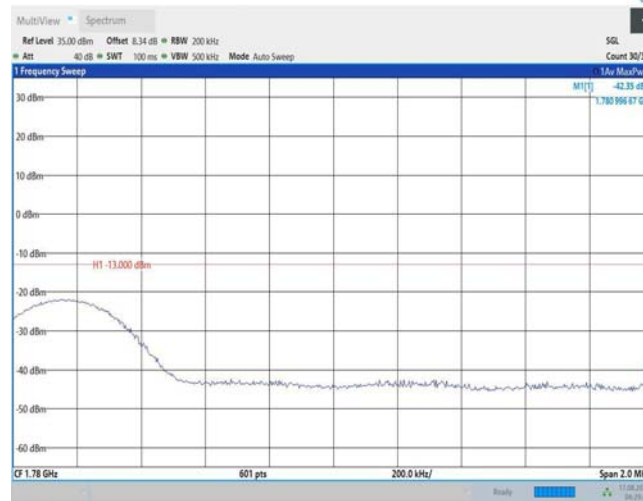
Band66-15MHz-QPSK-132597-1RB#74
