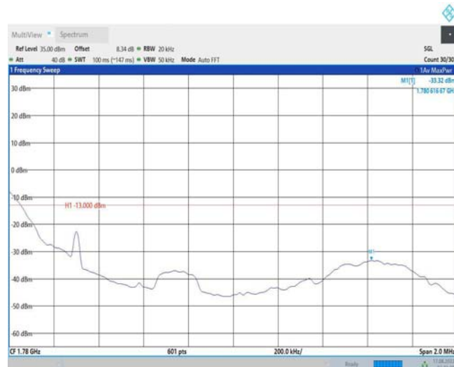
Band66-1.4MHz-QPSK-132665-1RB#5
