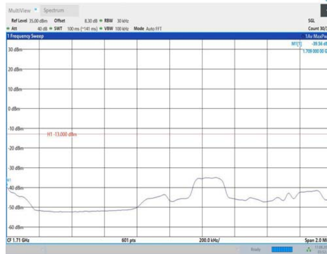
Band66-3MHz-16QAM-131987-15RB#0
