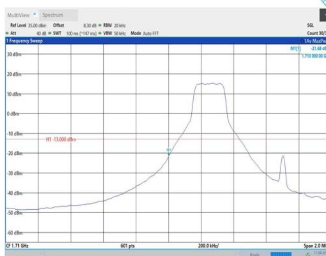
Band66-1.4MHz-16QAM-131979-1RB#5
