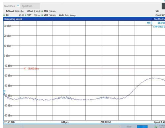
Band66-15MHz-16QAM-132597-1RB#0
