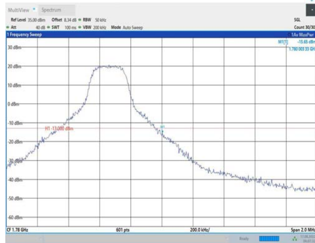
Band66-5MHz-QPSK-132647-25RB#0
