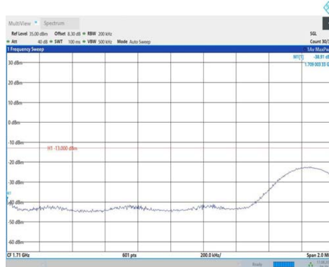
Band66-15MHz-QPSK-132047-75RB#0
