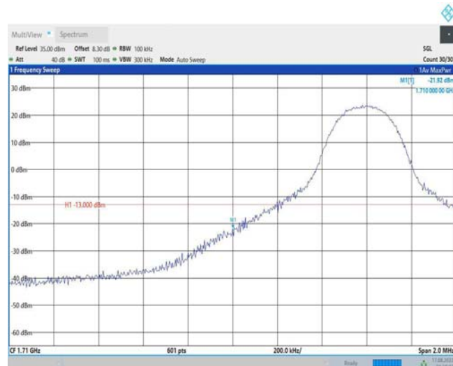
Band66-10MHz-16QAM-132022-1RB#49
