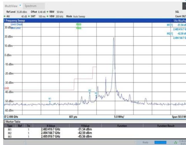
Band41-5MHz-16QAM-39675-25RB#0
