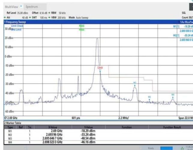
Band41-5MHz-16QAM-41565-25RB#0
