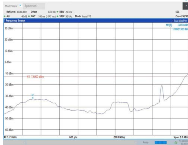
Band66-1.4MHz-16QAM-131979-6RB#0
