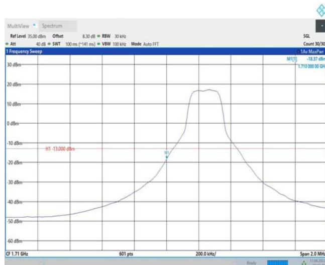
Band66-3MHz-16QAM-131987-1RB#14
