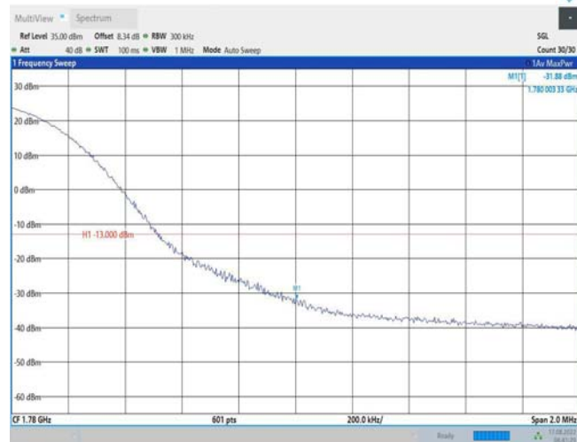
Band66-20MHz-16QAM-132572-1RB#99
