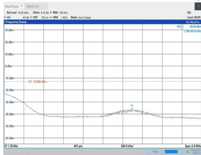
Band66-20MHz-16QAM-132572-1RB#99
