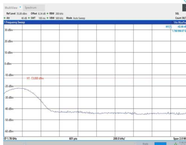
Band66-15MHz-16QAM-132597-1RB#74
