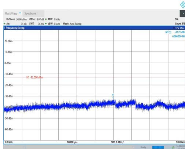
Band26-5MHz-QPSK-26740-1RB#0-Range1:30~1000MHz
