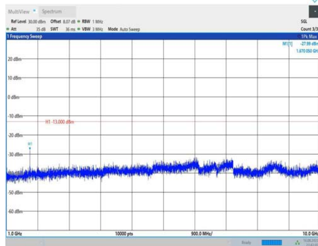
Band26-15MHz-QPSK-26965-1RB#0-Range2:1000~10000MHz
