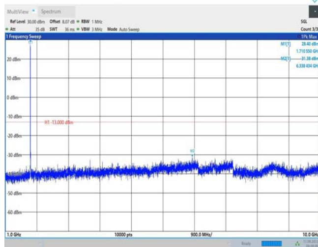
Band66-5MHz-QPSK-132322-1RB#0-Range1:30~1000MHz
