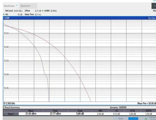
Band7-10MHz-QPSK-21400-50RB#0
