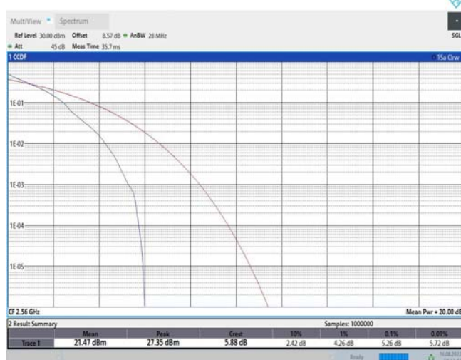
Band7-20MHz-QPSK-21350-100RB#0
