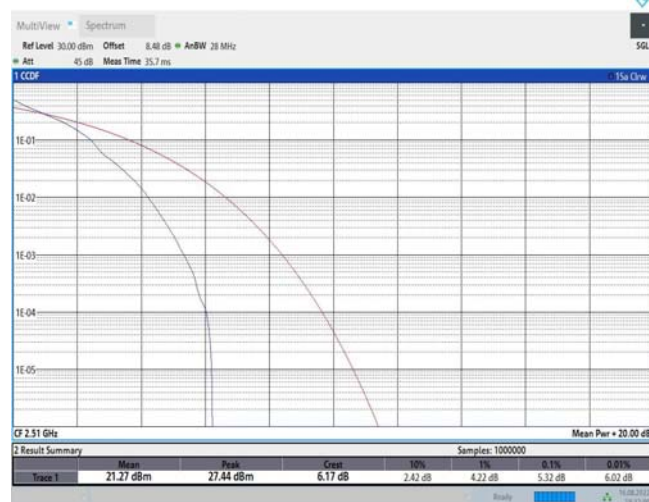
Band7-20MHz-QPSK-20850-100RB#0
