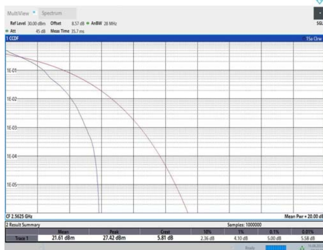
Band7-15MHz-QPSK-21375-75RB#0
