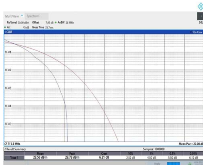
Band12-1.4MHz-QPSK-23173-6RB#0
