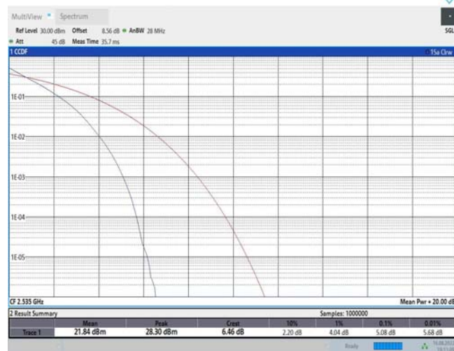
Band7-10MHz-QPSK-21400-1RB#0
