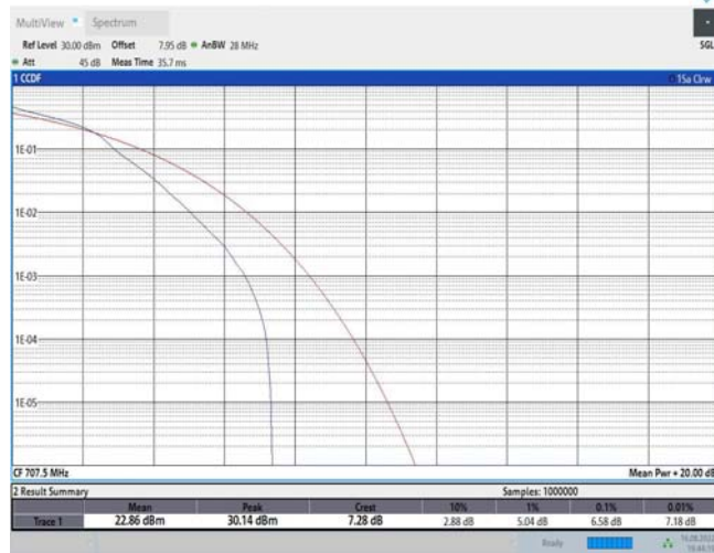
Band12-1.4MHz-16QAM-23095-6RB#0
