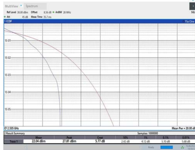
Band7-10MHz-QPSK-21100-50RB#0
