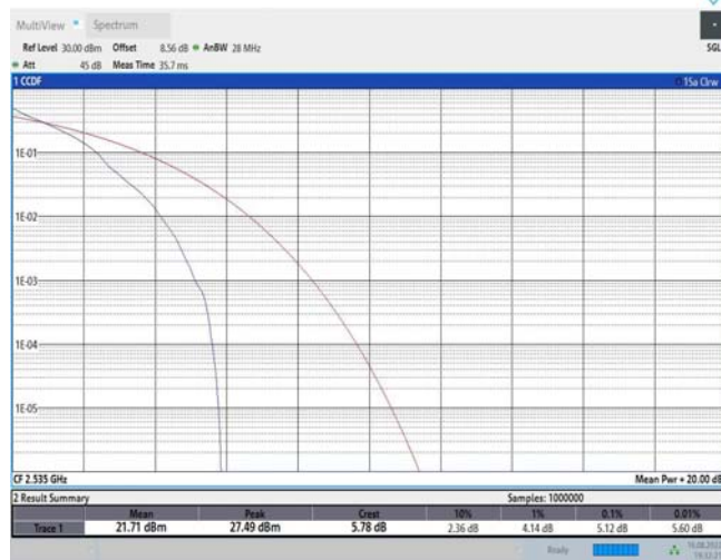
Band7-20MHz-QPSK-21100-100RB#0
