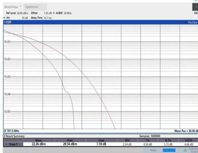
Band12-3MHz-QPSK-23095-15RB#0
