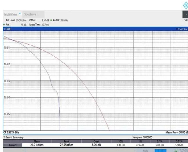
Band7-5MHz-QPSK-21425-25RB#0
