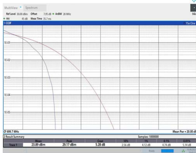
Band12-1.4MHz-QPSK-23017-6RB#0
