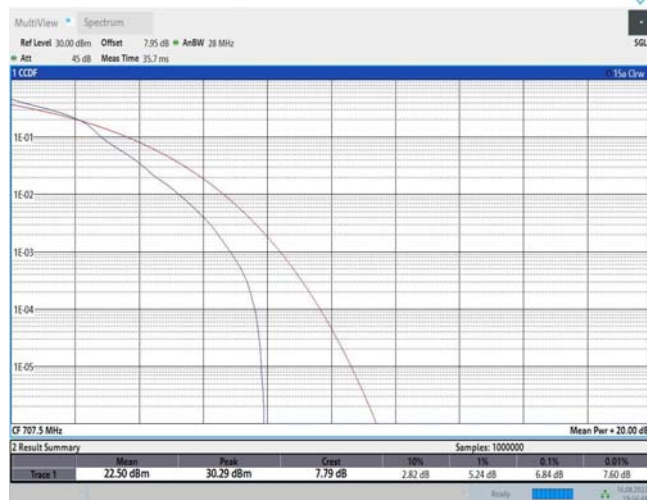
Band12-3MHz-16QAM-23095-15RB#0
