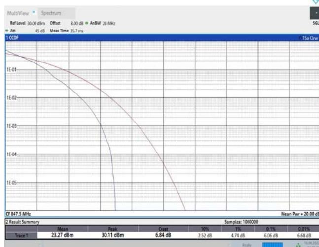
Band26-3MHz-QPSK-27025-15RB#0
