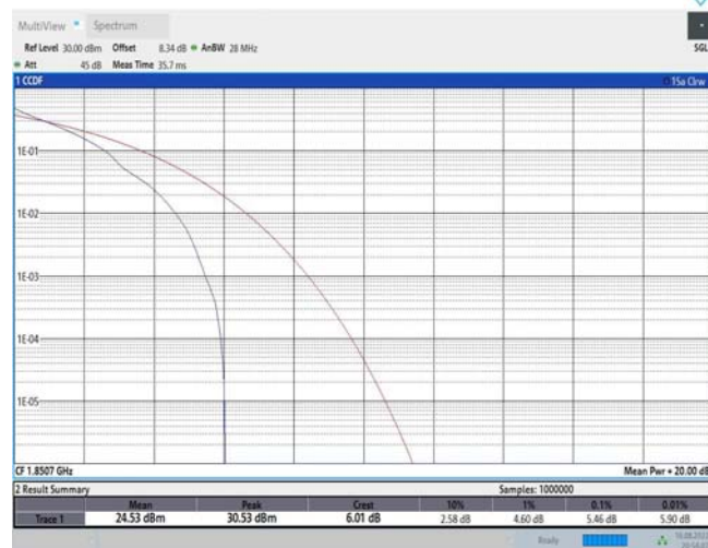
Band25-1.4MHz-QPSK-26047-6RB#0
