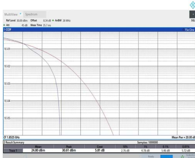
Band25-5MHz-16QAM-26065-25RB#0
