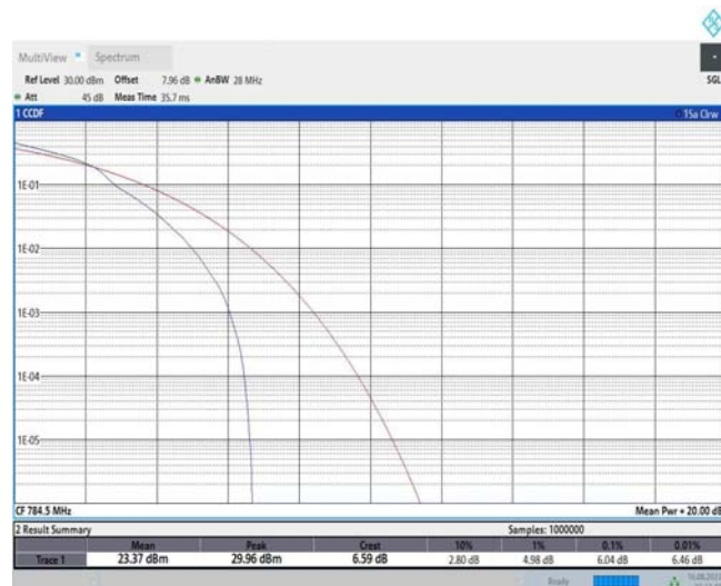
Band13-5MHz-16QAM-23255-25RB#0
