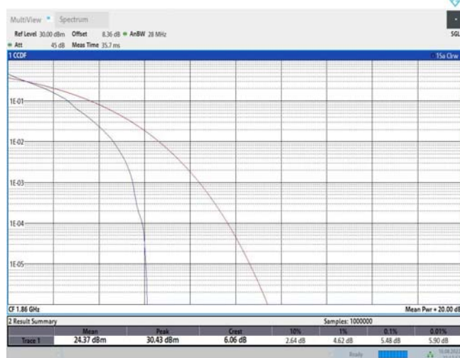
Band25-20MHz-QPSK-26140-100RB#0
