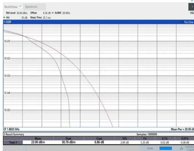
Band25-5MHz-16QAM-26365-25RB#0
