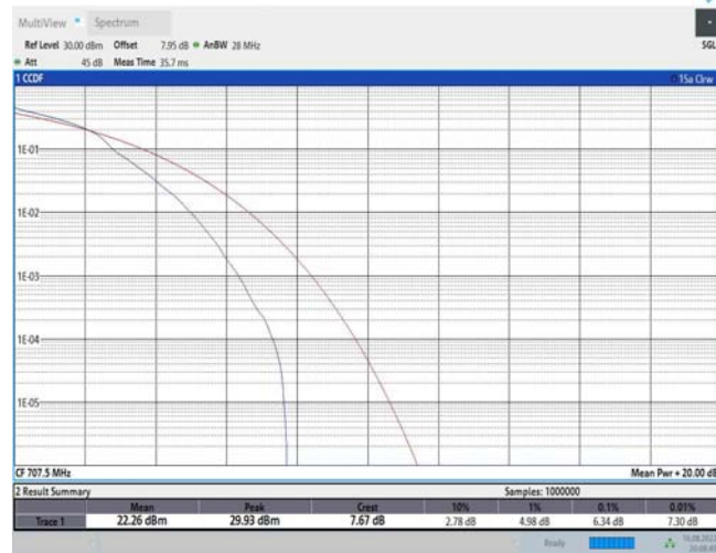
Band12-5MHz-16QAM-23095-25RB#0
