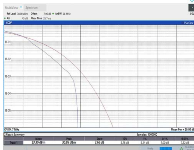
Band26-1.4MHz-16QAM-26697-6RB#0
