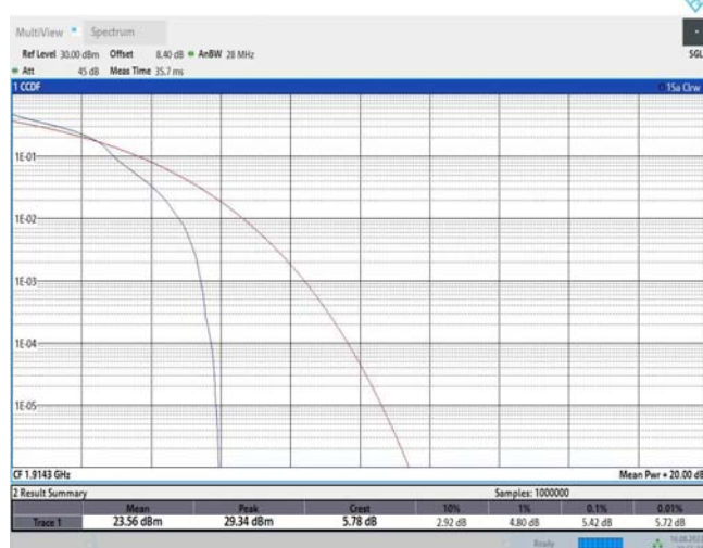
Band25-1.4MHz-16QAM-26683-6RB#0
