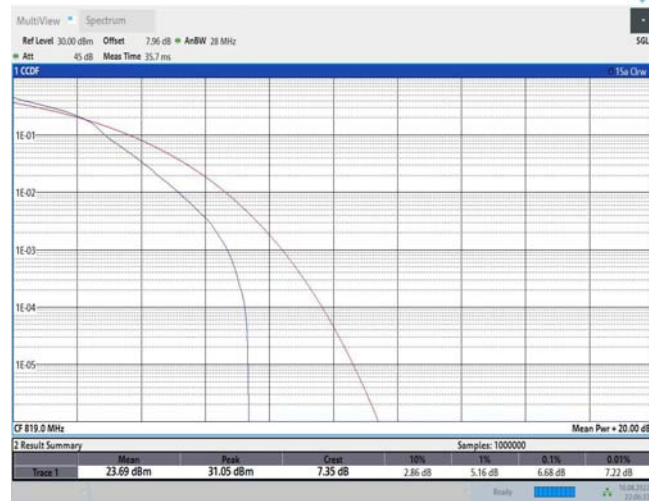
Band26-1.4MHz-16QAM-26740-6RB#0
