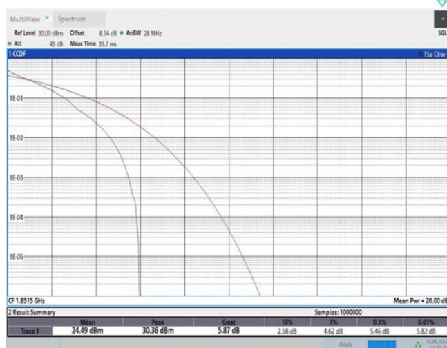
Band25-3MHz-QPSK-26055-15RB#0
