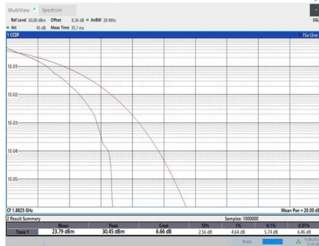
Band25-15MHz-QPSK-26365-75RB#0
