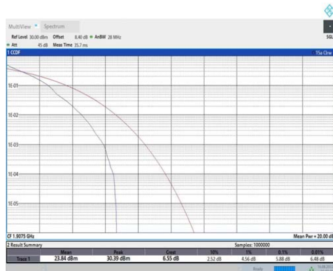
Band25-15MHz-QPSK-26615-75RB#0
