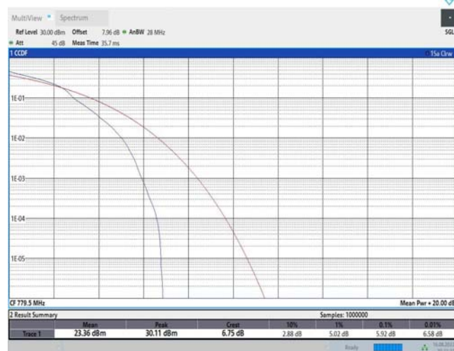
Band13-5MHz-16QAM-23205-25RB#0
