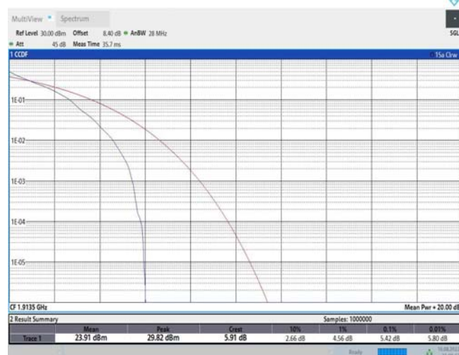
Band25-3MHz-QPSK-26675-15RB#0
