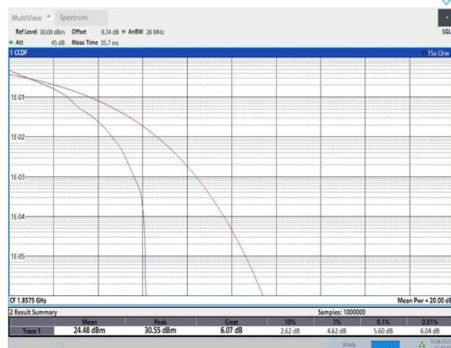
Band25-15MHz-QPSK-26115-75RB#0
