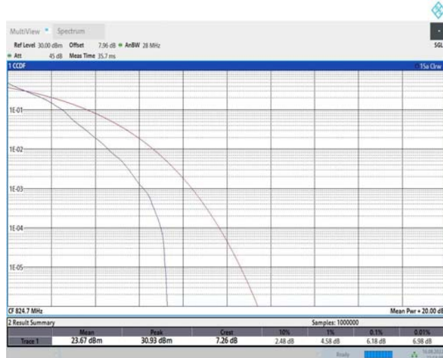
Band26-1.4MHz-QPSK-26797-6RB#0
