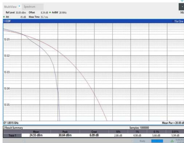
Band25-3MHz-16QAM-26055-15RB#0
