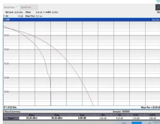
Band25-5MHz-QPSK-26665-25RB#0
