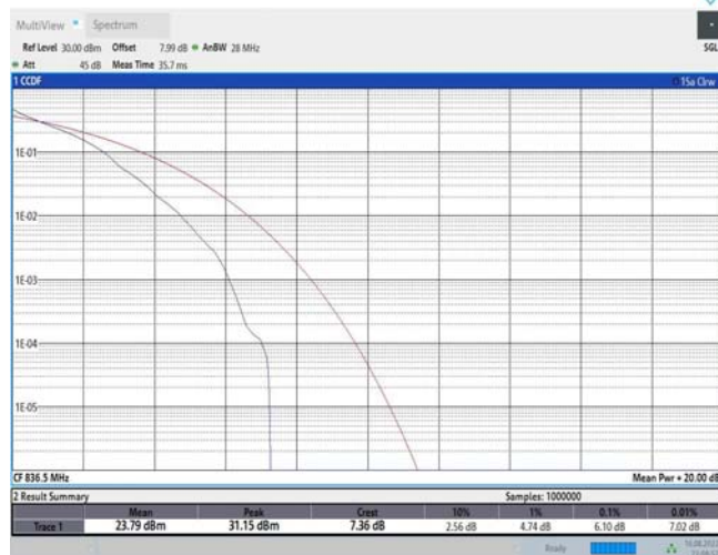
Band26-3MHz-QPSK-26915-15RB#0
