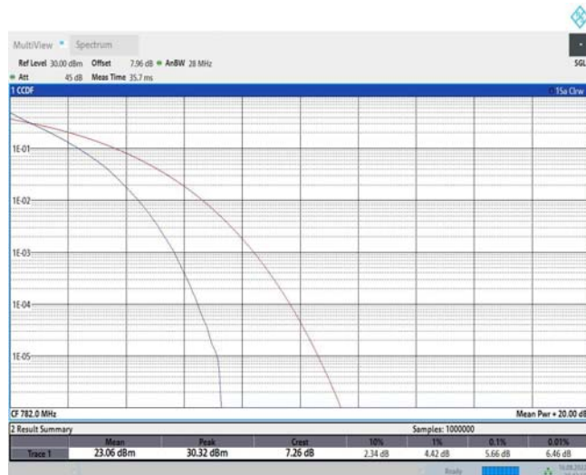
Band13-10MHz-16QAM-23230-1RB#0
