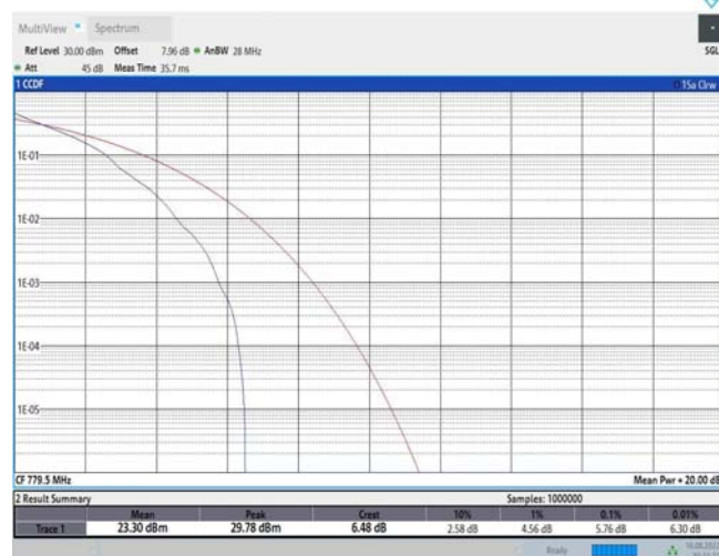
Band13-5MHz-QPSK-23205-25RB#0
