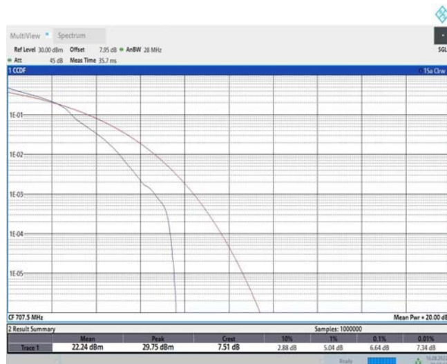
Band12-10MHz-16QAM-23130-1RB#0
