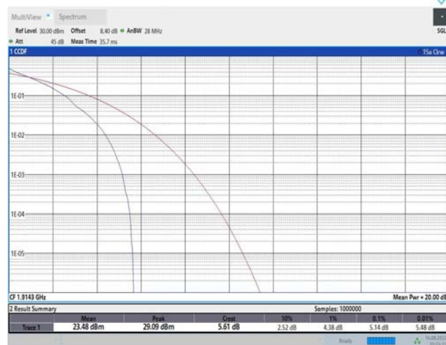
Band25-1.4MHz-QPSK-26683-6RB#0
