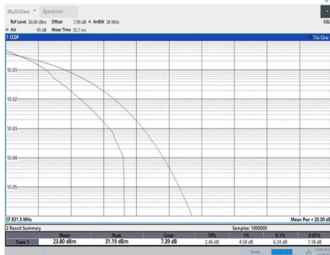
Band26-15MHz-QPSK-26865-75RB#0
