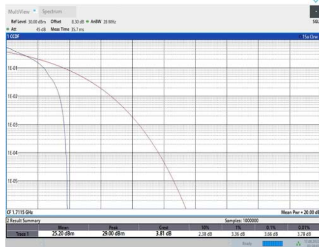
Band66-3MHz-QPSK-131987-15RB#0
