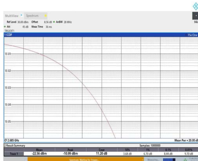
Band41-10MHz-QPSK-41540-50RB#0
