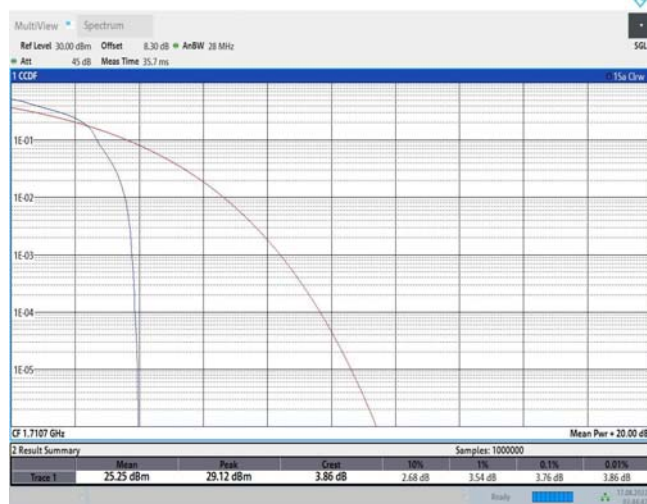
Band66-1.4MHz-16QAM-131979-6RB#0
