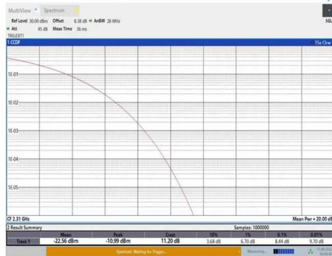
Band40-5MHz-16QAM-38750-25RB#0
