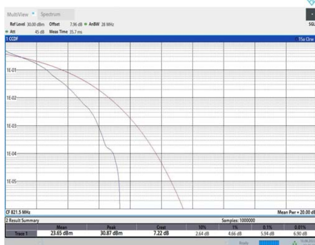
Band26-5MHz-QPSK-26765-25RB#0
