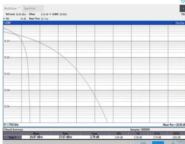
Band66-1.4MHz-QPSK-132665-6RB#0
