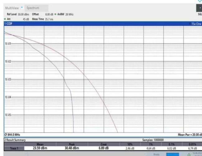
Band26-10MHz-QPSK-26990-50RB#0
