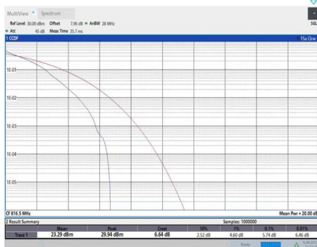
Band26-5MHz-QPSK-26715-25RB#0
