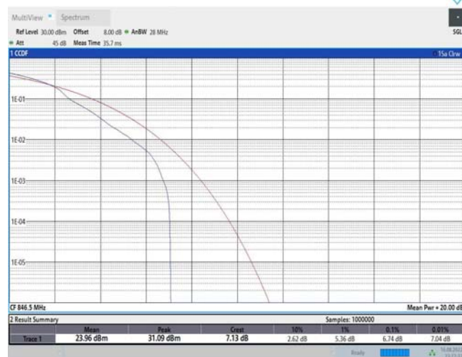
Band26-5MHz-16QAM-27015-25RB#0
