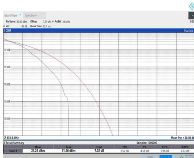
Band26-10MHz-QPSK-26915-50RB#0
