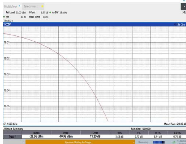
Band41-20MHz-QPSK-40620-100RB#0
