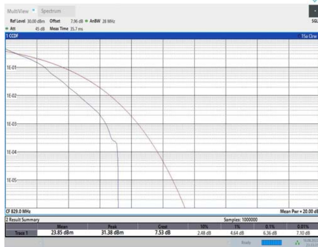
Band26-10MHz-QPSK-26840-50RB#0
