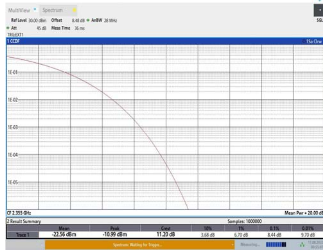
Band40-5MHz-16QAM-39200-25RB#0
