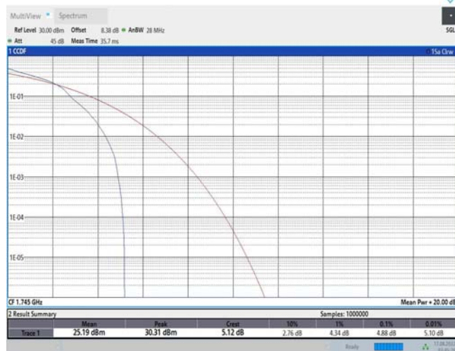
Band66-1.4MHz-16QAM-132322-6RB#0
