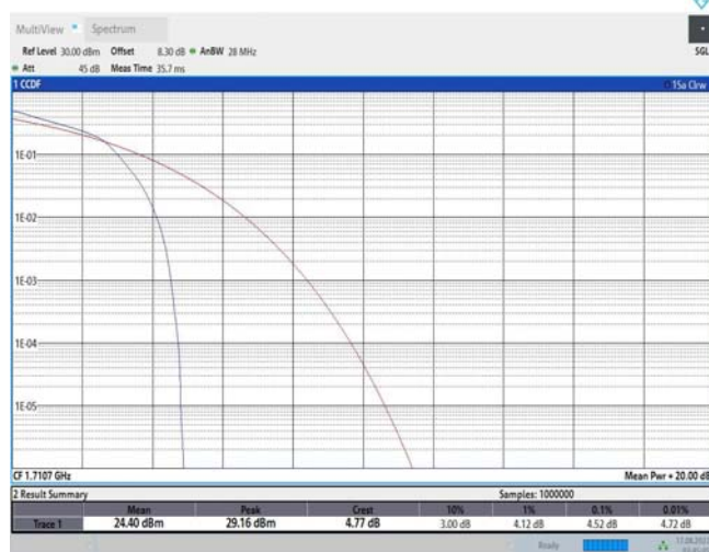
Band66-1.4MHz-16QAM-132322-1RB#0
