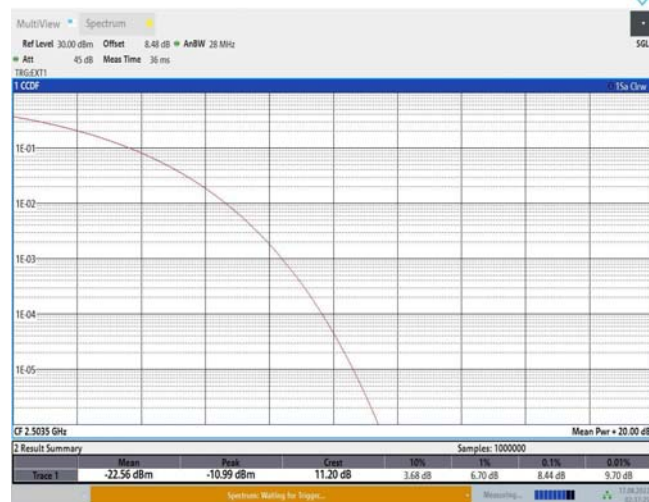
Band41-15MHz-QPSK-39725-75RB#0
