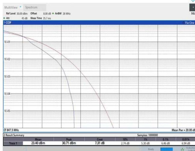
Band26-3MHz-16QAM-27025-15RB#0
