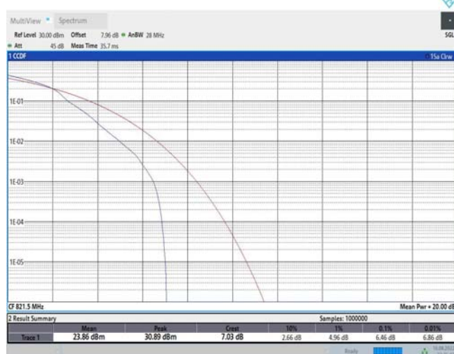
Band26-5MHz-16QAM-26765-25RB#0
