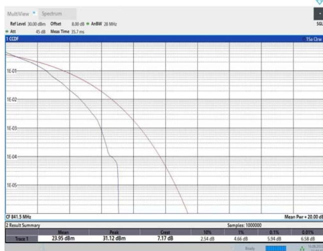
Band26-15MHz-QPSK-26965-75RB#0
