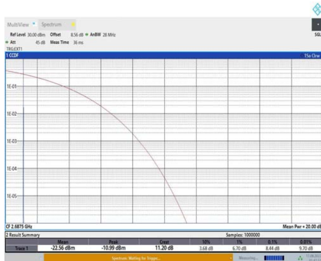
Band41-5MHz-16QAM-41565-25RB#0
