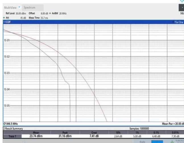
Band26-5MHz-QPSK-27015-25RB#0
