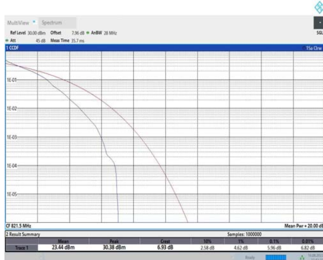
Band26-15MHz-QPSK-26765-75RB#0
