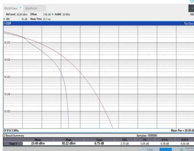
Band26-5MHz-16QAM-26715-25RB#0
