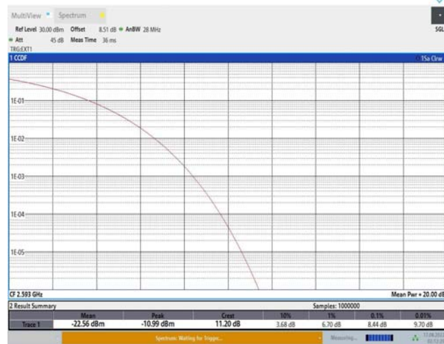
Band41-10MHz-QPSK-40620-50RB#0
