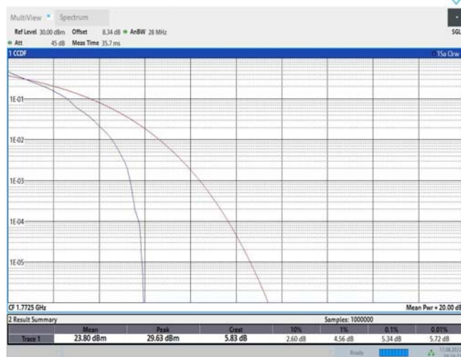
Band66-15MHz-QPSK-132597-75RB#0
