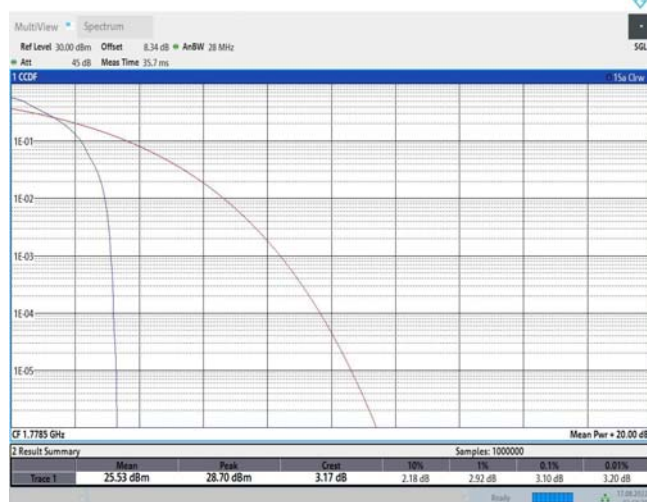
Band66-3MHz-QPSK-132657-15RB#0
