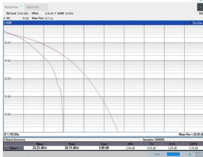
Band66-20MHz-QPSK-132322-100RB#0
