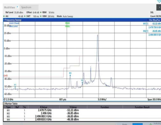
Band7-5MHz-16QAM-20775-25RB#0
