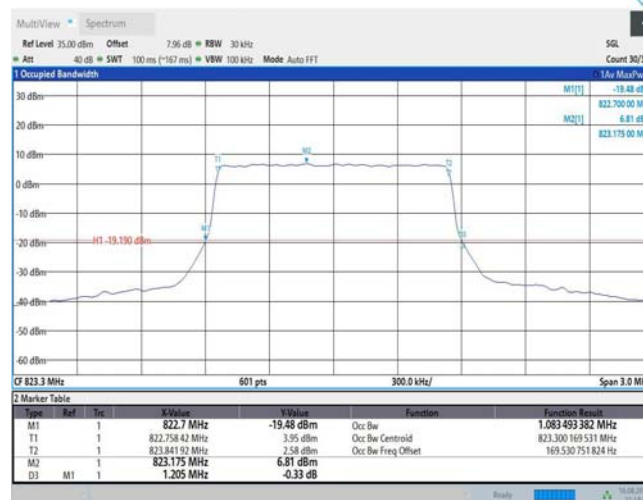
Band26-1.4MHz-16QAM-26797-6RB#0
