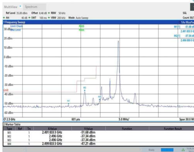
Band7-5MHz-QPSK-20775-25RB#0
