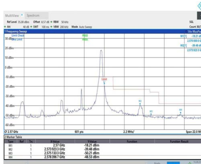
Band7-5MHz-QPSK-21425-25RB#0
