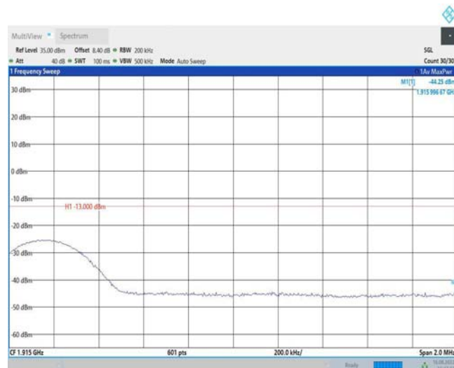
Band25-15MHz-QPSK-26615-1RB#74
