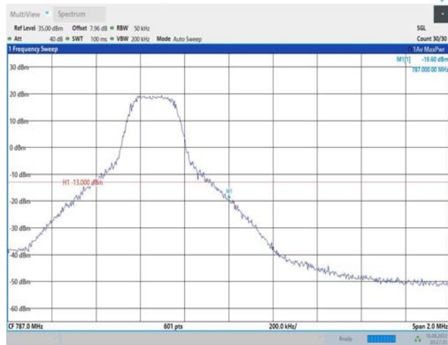
Band13-5MHz-16QAM-23255-25RB#0
