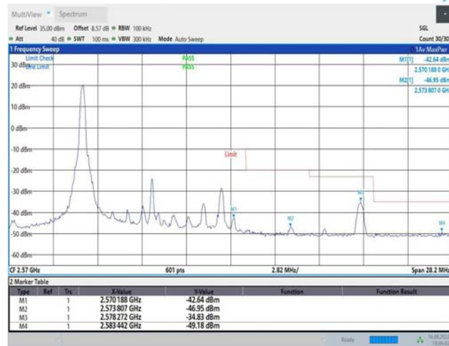
Band7-10MHz-16QAM-21400-1RB#49
