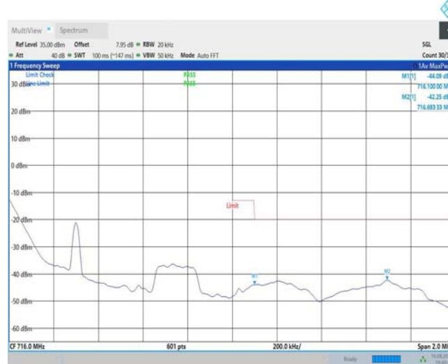
Band12-1.4MHz-16QAM-23173-1RB#5
