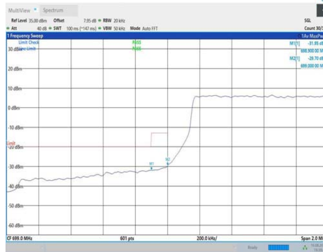
Band12-1.4MHz-QPSK-23173-1RB#0
