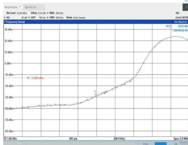
Band25-15MHz-QPSK-26115-1RB#74
