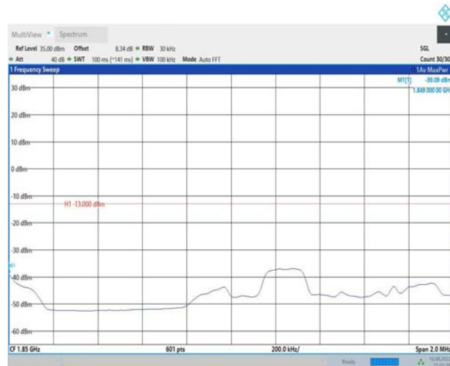
Band25-3MHz-16QAM-26055-15RB#0
