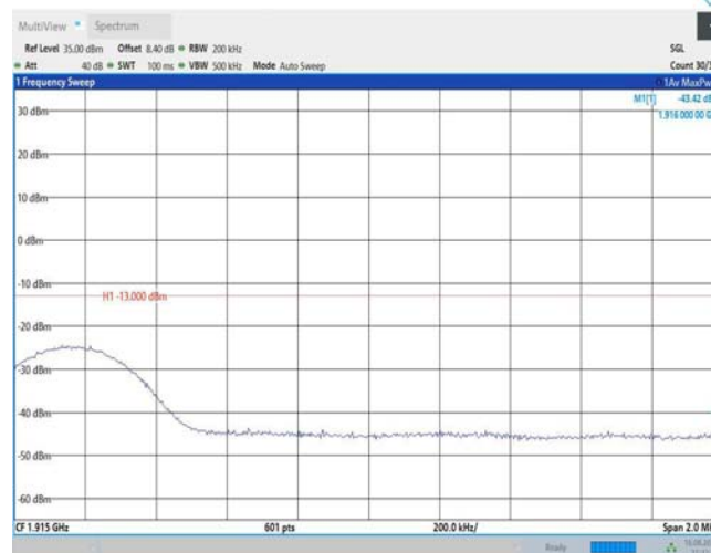
Band25-15MHz-16QAM-26615-1RB#74
