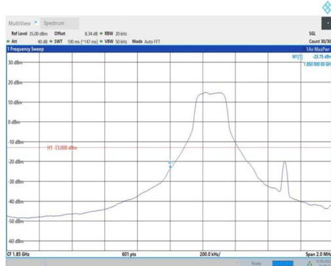
Band25-1.4MHz-QPSK-26047-1RB#5
