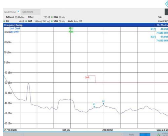
Band12-1.4MHz-QPSK-23173-1RB#5
