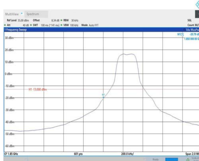
Band25-3MHz-QPSK-26055-1RB#14
