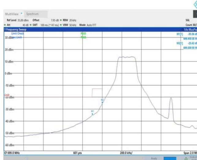
Band12-1.4MHz-16QAM-23017-1RB#5
