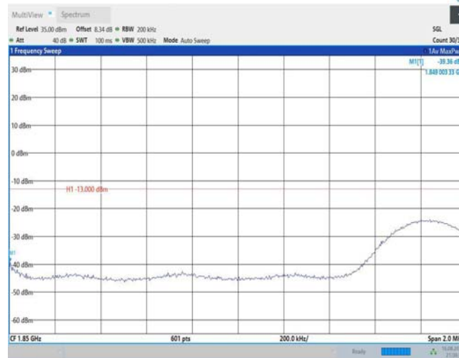
Band25-15MHz-16QAM-26615-1RB#0
