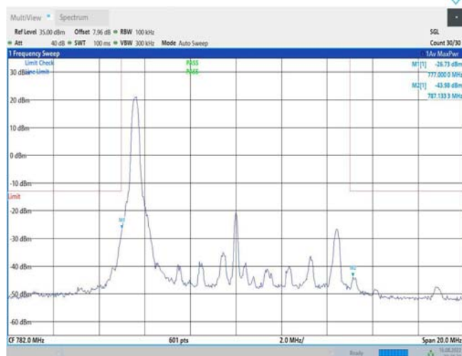
Band13-10MHz-QPSK-23230-1RB#49
