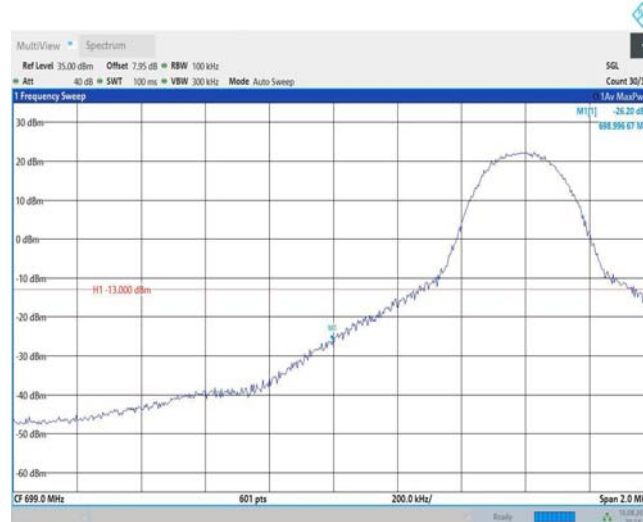
Band12-10MHz-QPSK-23060-1RB#49
