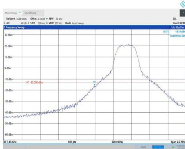
Band25-5MHz-16QAM-26065-1RB#24
