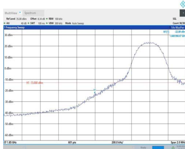
Band25-10MHz-16QAM-26090-1RB#49
