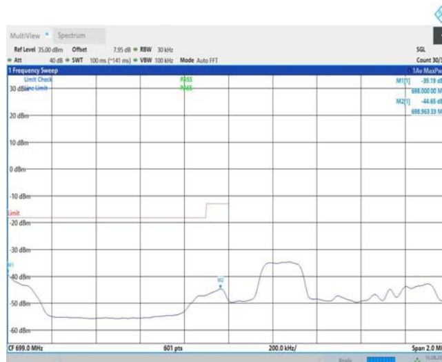
Band12-3MHz-QPSK-23025-15RB#0
