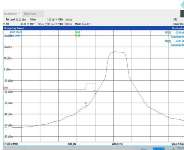
Band12-3MHz-QPSK-23025-1RB#14
