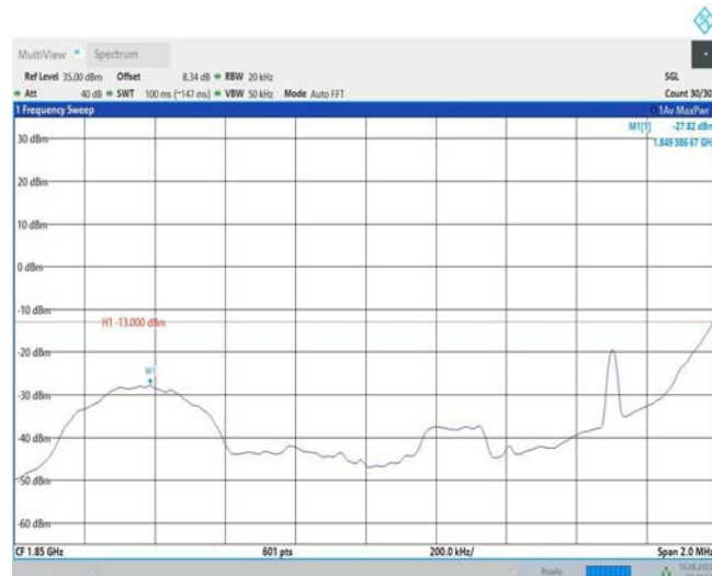
Band25-1.4MHz-QPSK-26047-6RB#0
