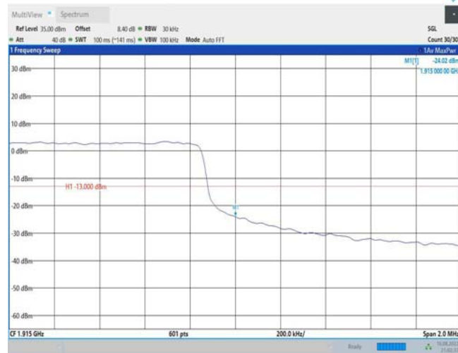
Band25-3MHz-16QAM-26055-1RB#0
