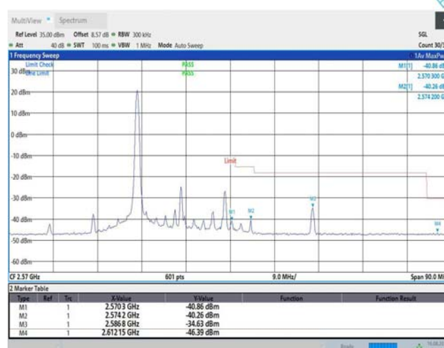
Band7-20MHz-16QAM-21350-1RB#99
