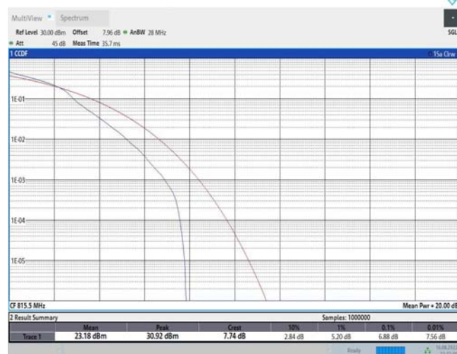
Band26-3MHz-16QAM-26705-15RB#0
