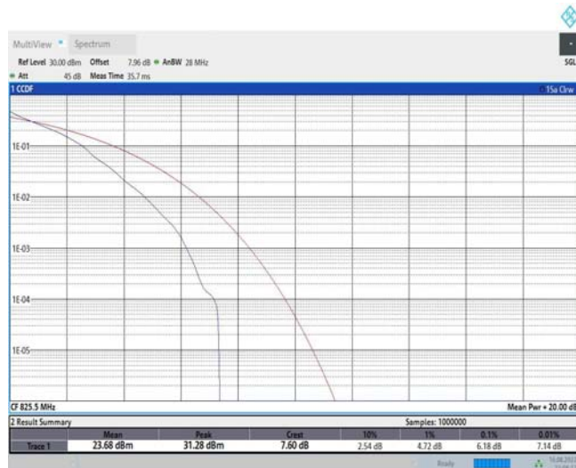
Band26-3MHz-QPSK-26805-15RB#0
