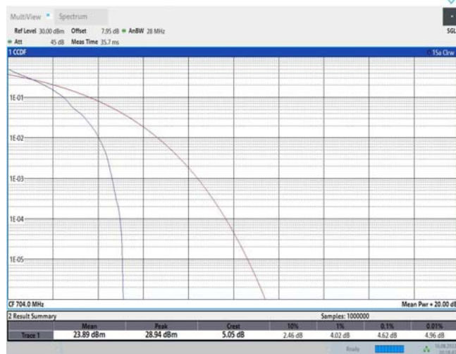
Band12-10MHz-QPSK-23060-50RB#0
