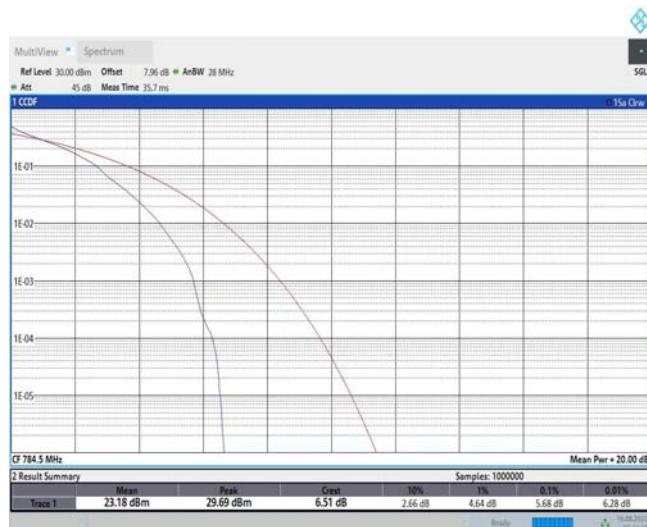
Band13-5MHz-QPSK-23255-25RB#0
