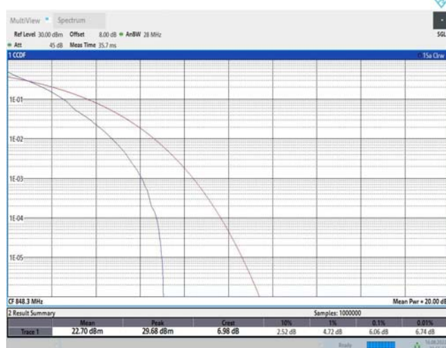
Band26-1.4MHz-QPSK-27033-6RB#0
