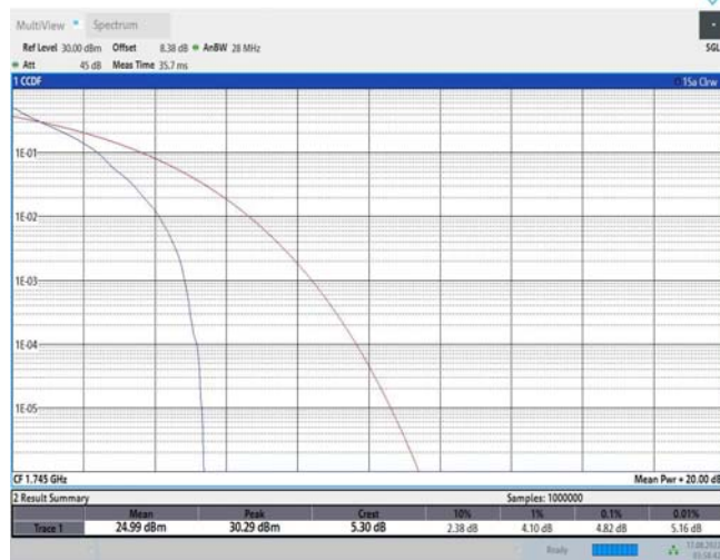
Band66-3MHz-QPSK-132322-15RB#0
