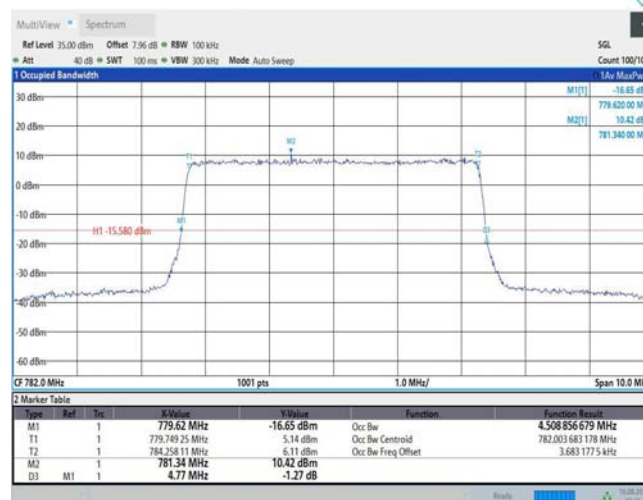
Band13-5MHz-16QAM-23255-25RB#0
