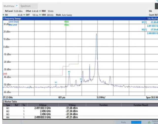
Band7-5MHz-QPSK-20775-25RB#0
