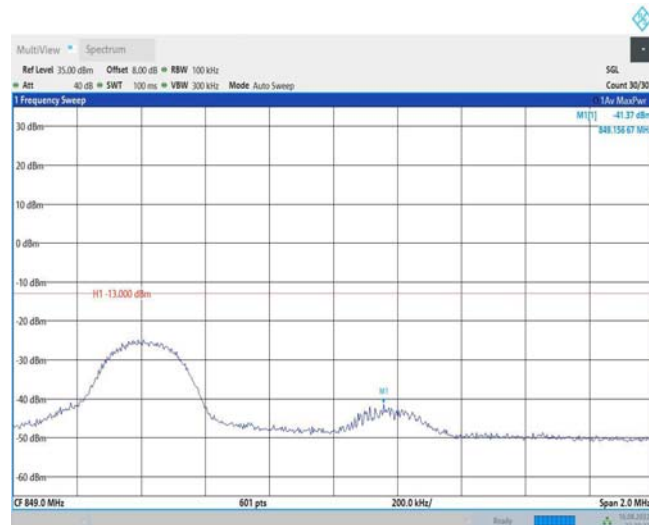
Band26-10MHz-16QAM-26990-1RB#49
