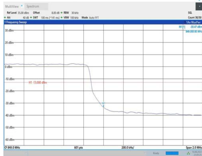
Band26-3MHz-16QAM-26705-1RB#0
