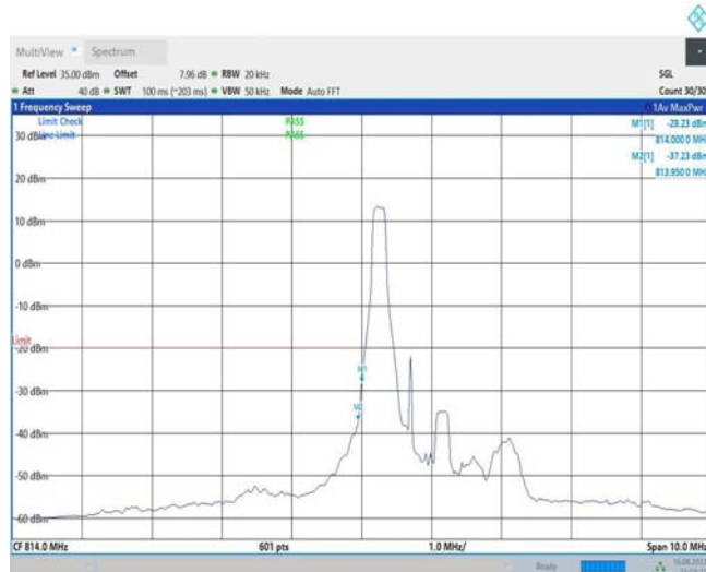
Band26-1.4MHz-QPSK-26697-1RB#5
