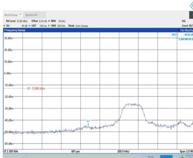
Band40-5MHz-16QAM-38725-25RB#0
