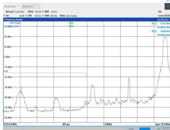
Band26-5MHz-16QAM-26715-25RB#0
