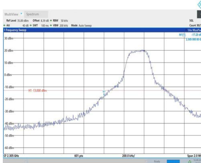
Band40-5MHz-16QAM-38725-1RB#24
