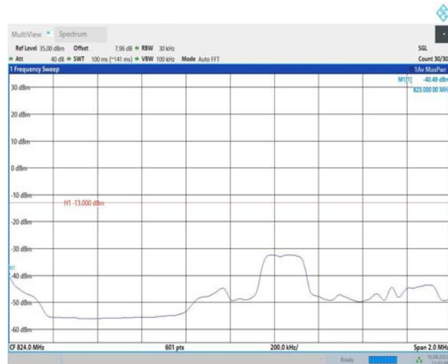
Band26-3MHz-16QAM-26805-15RB#0
