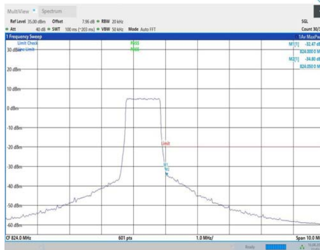
Band26-1.4MHz-16QAM-26797-1RB#0
