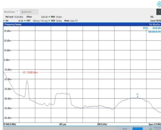
Band26-1.4MHz-16QAM-27033-1RB#5
