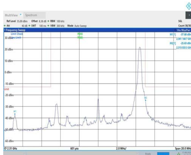
Band40-10MHz-QPSK-38750-50RB#0
