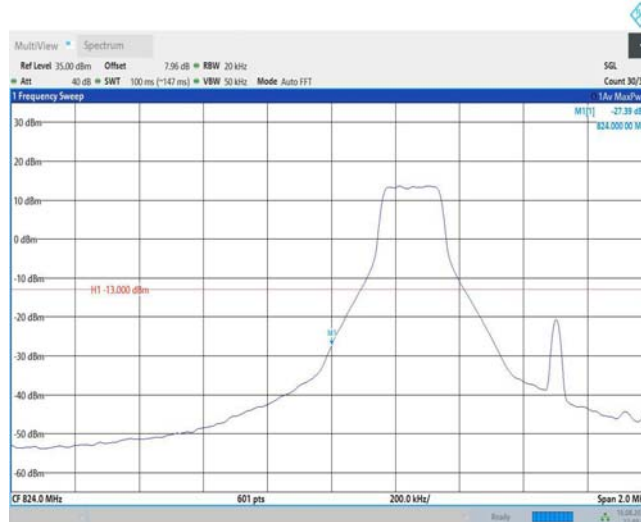
Band26-1.4MHz-16QAM-26797-1RB#5
