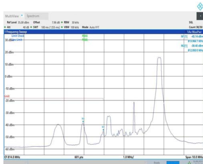
Band26-3MHz-16QAM-26705-15RB#0
