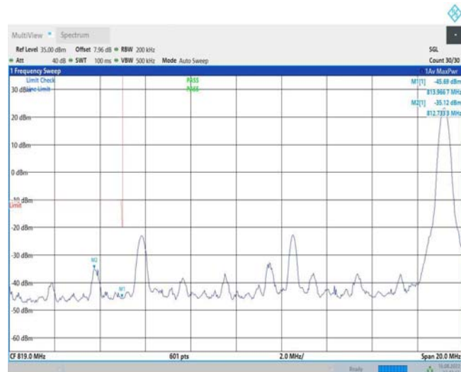
Band26-15MHz-QPSK-26765-75RB#0
