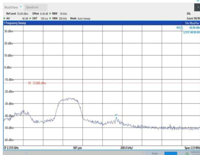
Band40-5MHz-QPSK-38775-1RB#24
