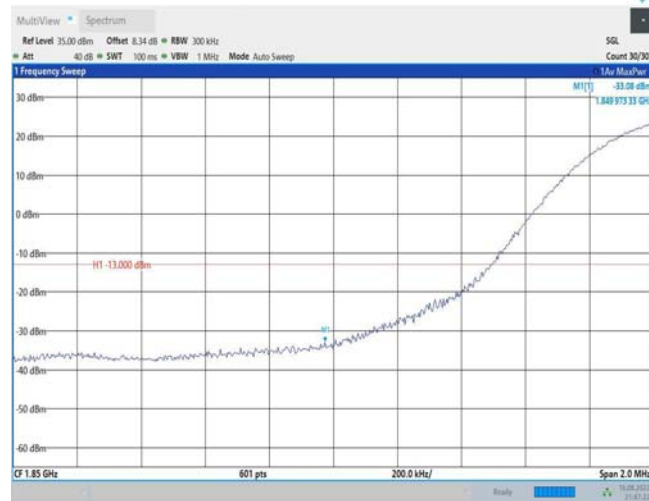
Band25-20MHz-16QAM-26140-1RB#99
