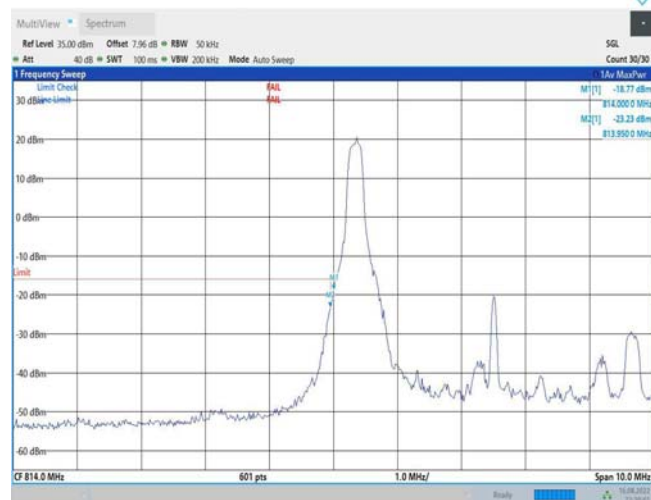
Band26-5MHz-16QAM-26715-1RB#24
