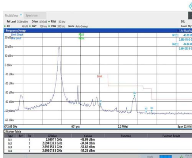
Band41-5MHz-QPSK-41565-1RB#24
