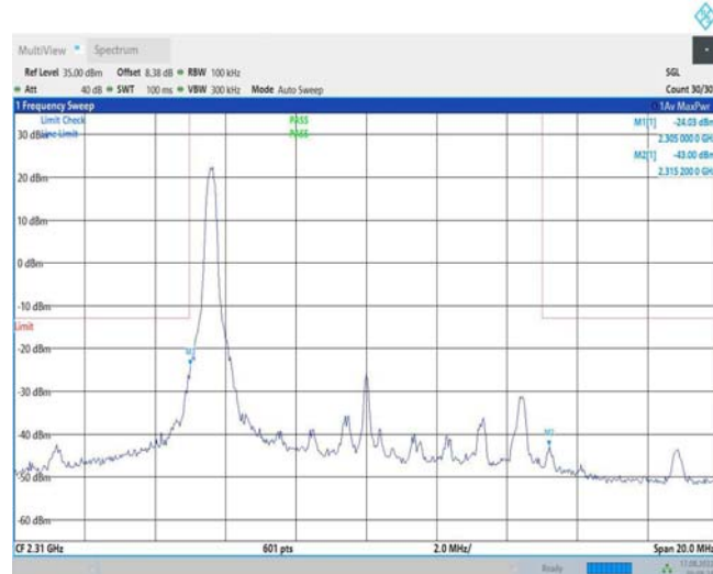
Band40-10MHz-QPSK-38750-1RB#49
