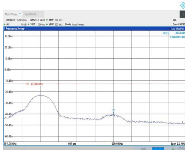
Band66-10MHz-QPSK-132622-1RB#49
