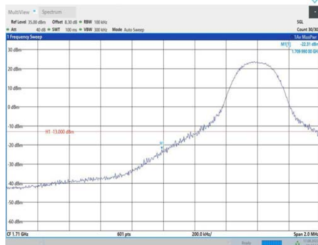
Band66-10MHz-QPSK-132022-1RB#49
