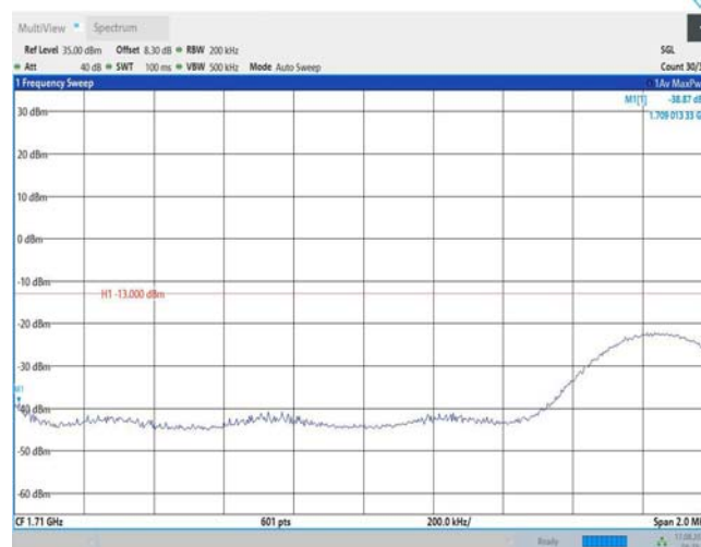
Band66-15MHz-16QAM-132597-1RB#0
