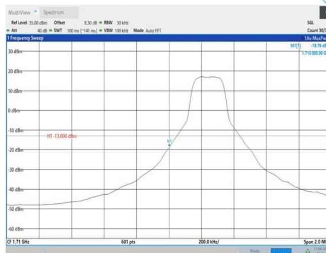
Band66-3MHz-QPSK-131987-1RB#14
