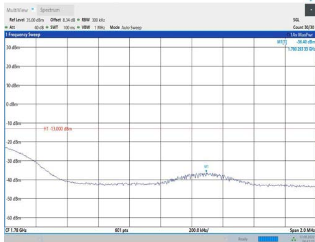
Band66-20MHz-16QAM-132572-1RB#99
