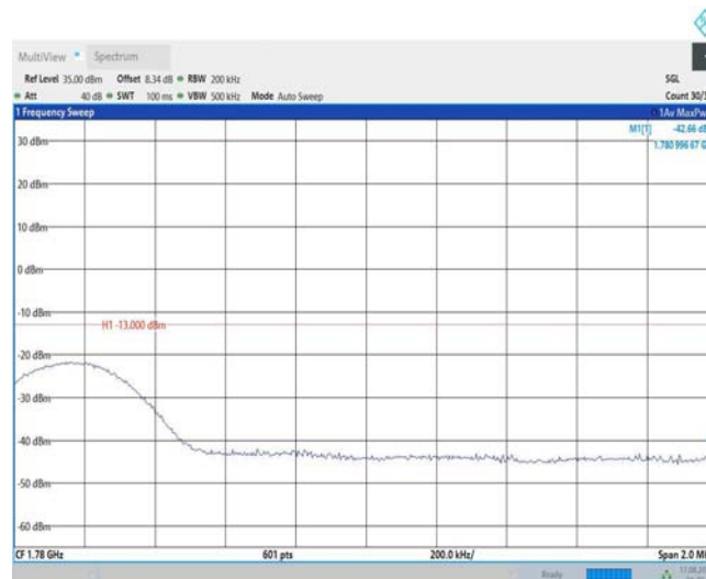
Band66-15MHz-16QAM-132597-1RB#74
