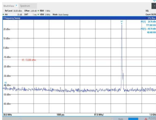
Band13-5MHz-QPSK-23205-1RB#0-Range1:30~1000MHz
