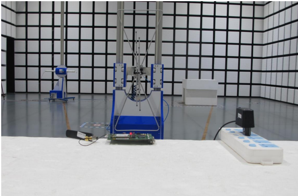
RSE (30MHz-1GHz)
