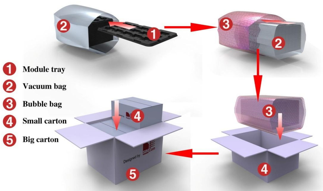
Figure 37: packaging diagram
