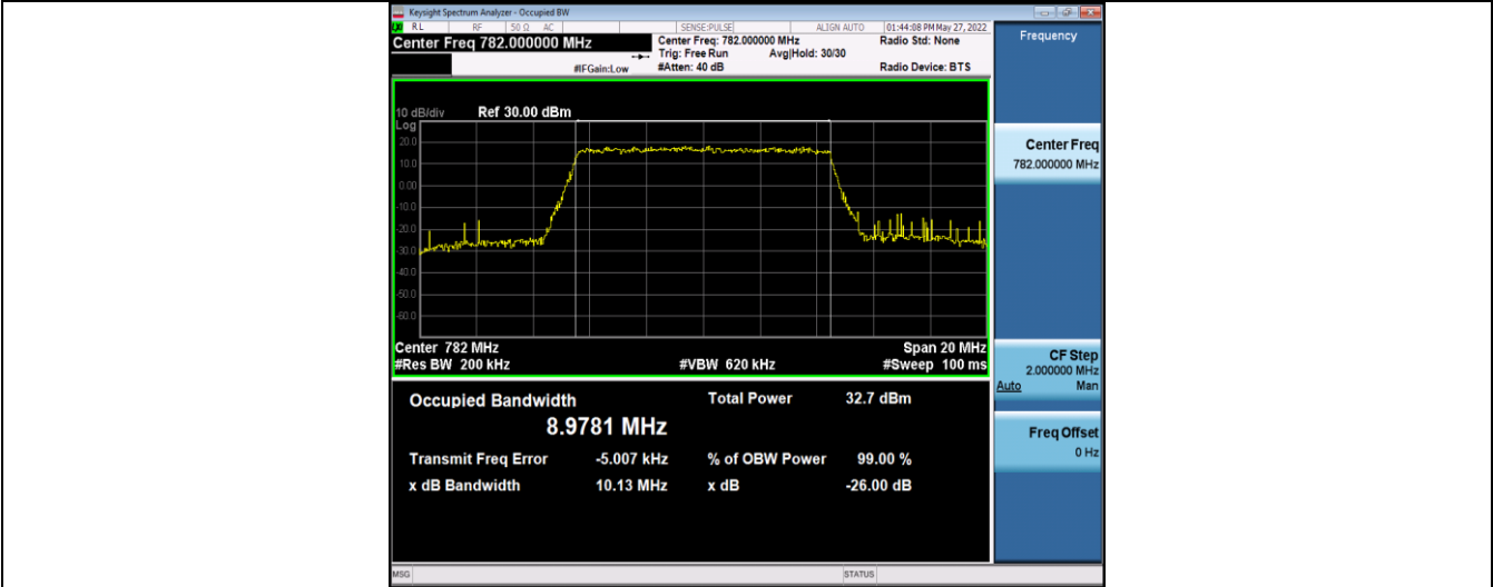
Band13-10MHz-16QAM-23230-50RB#0
