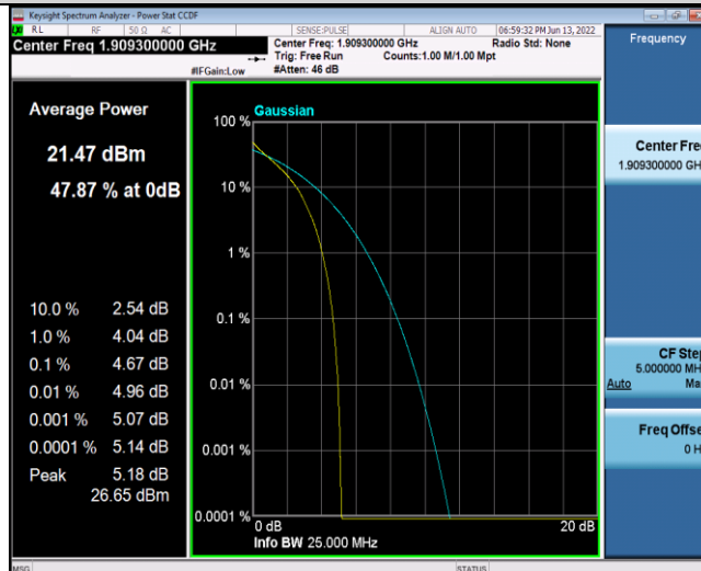
Band2-1.4MHz-QPSK-19193-25RB#0
