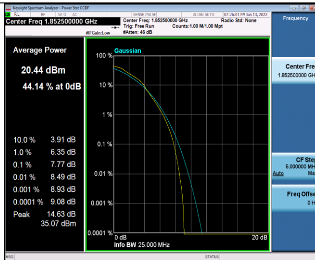
Band2-5MHz-16QAM-185250000-25RB#0
