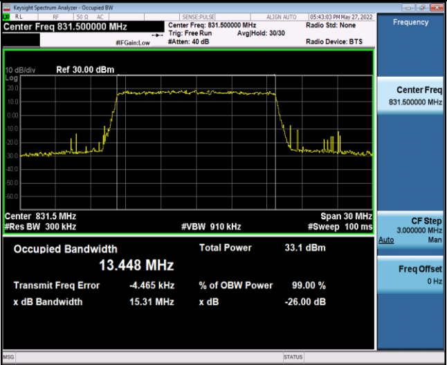
Band26-15MHz-QPSK-26915-75RB#0
