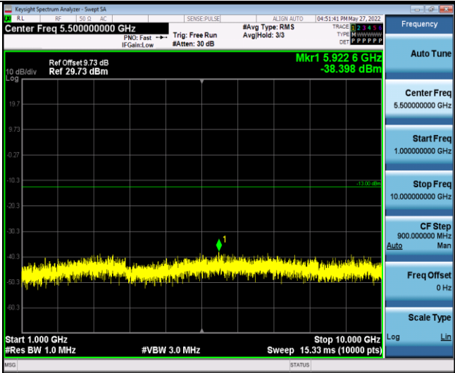
Band26-1.4MHz-16QAM-26697-6RB#0-Range1:30~1000MHz
