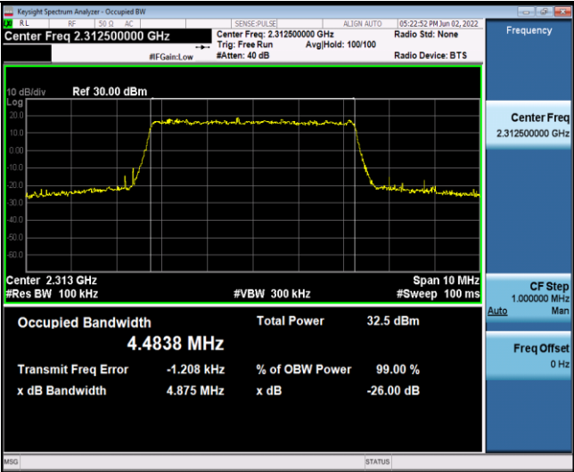
Band30-5MHz-16QAM-27685-25RB#0
