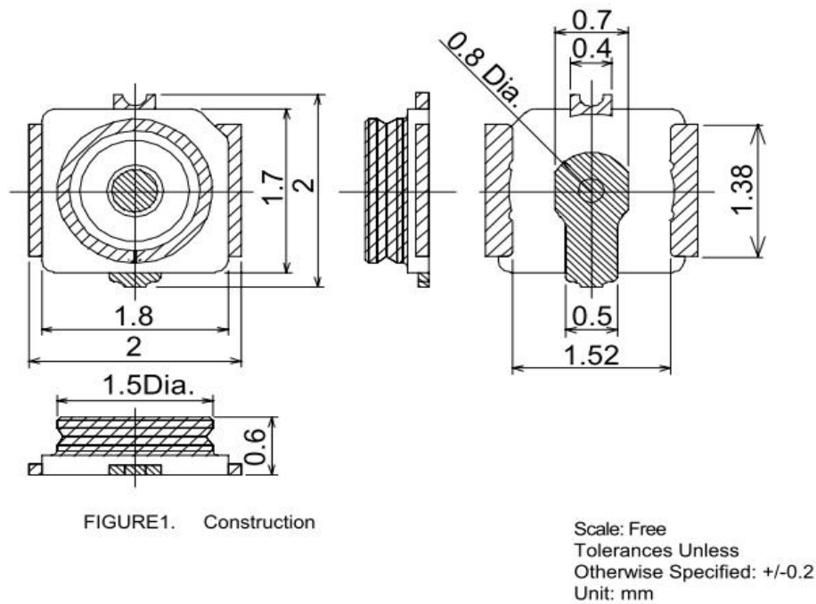
Figure 21: Antenna connector
