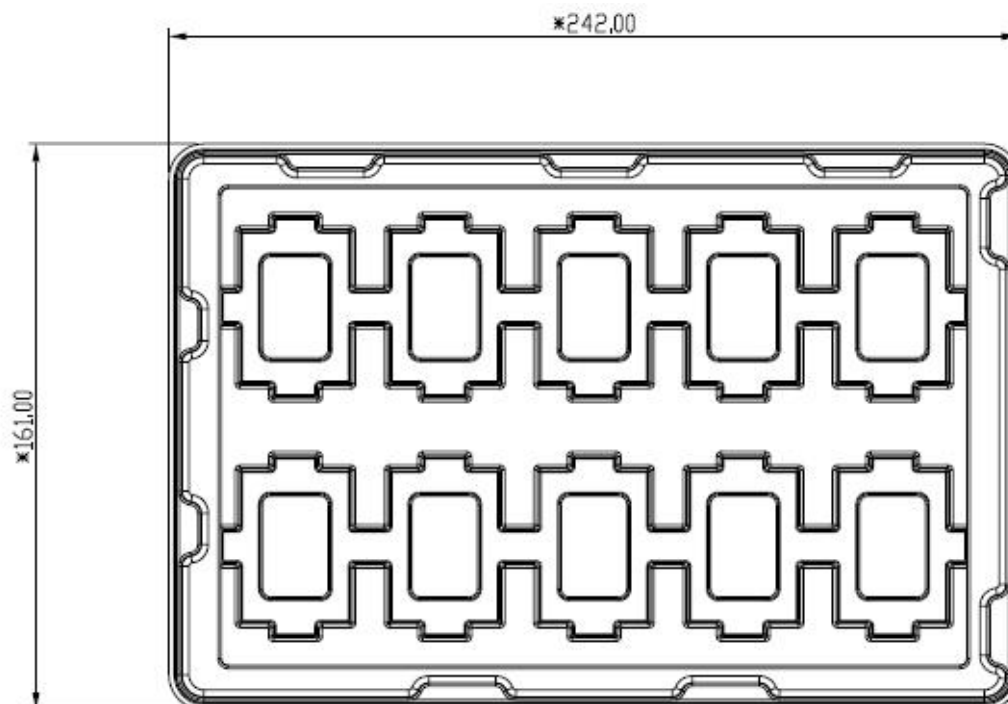
Figure 24: Tray drawing
