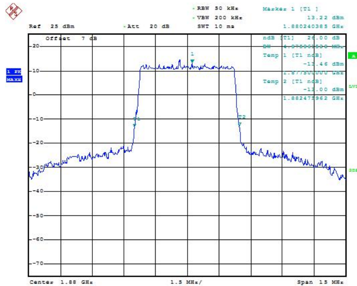
Fig.45 LTE band 2, 5MHz Bandwidth, QPSK (-26dBc BW)
