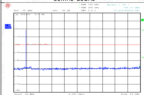
Conducted spurious emission: Ch39, 30MHz~26GHz
