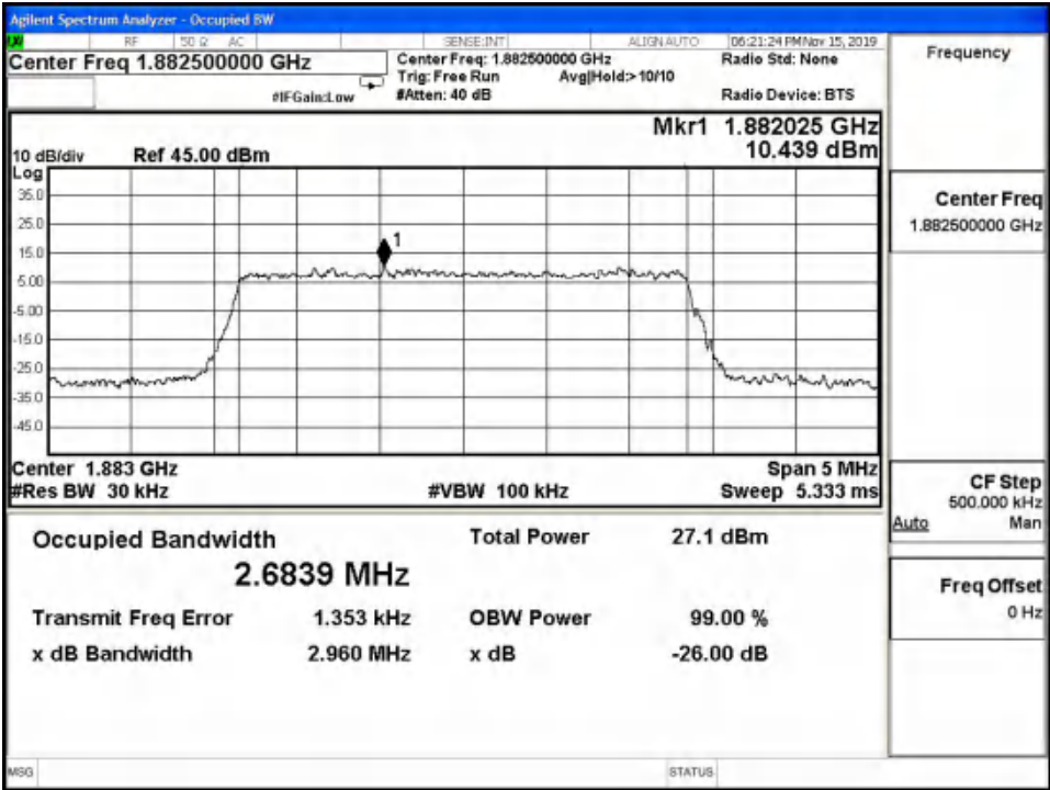
LTE Band25 QPSK 99% Channel 26365 BW=3MHz RB=15 RB Offset=0
