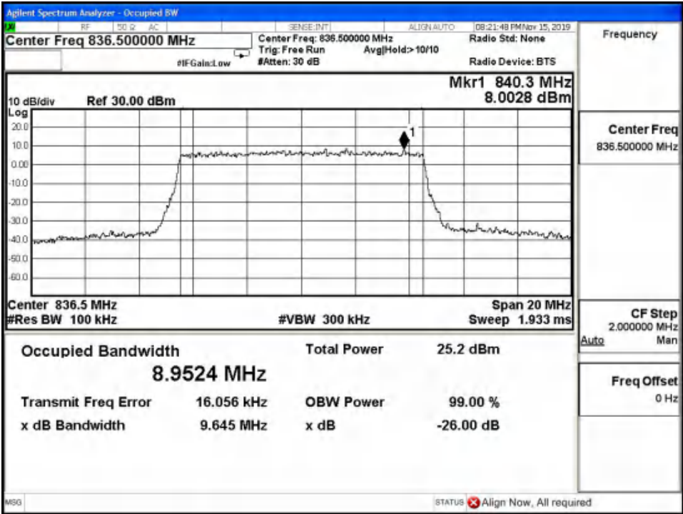
LTE Band26 16QAM 99% Channel 26915 BW=10MHz RB=50 RB Offset=0
