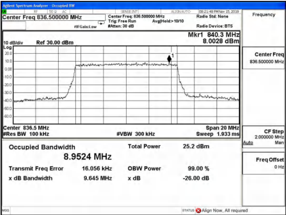
LTE Band26 16QAM -26dBc Channel 26915 BW=10MHz RB=50 RB Offset=0
