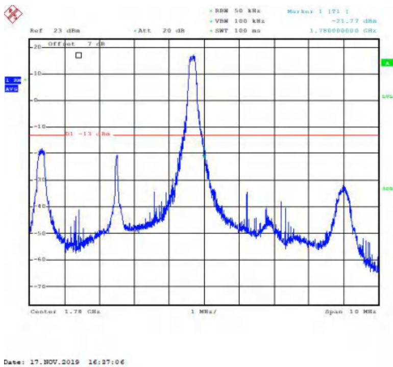
LTE Band66, 5MHz bandwidth, QPSK,(1,25) Mode, Above 1780MHz
