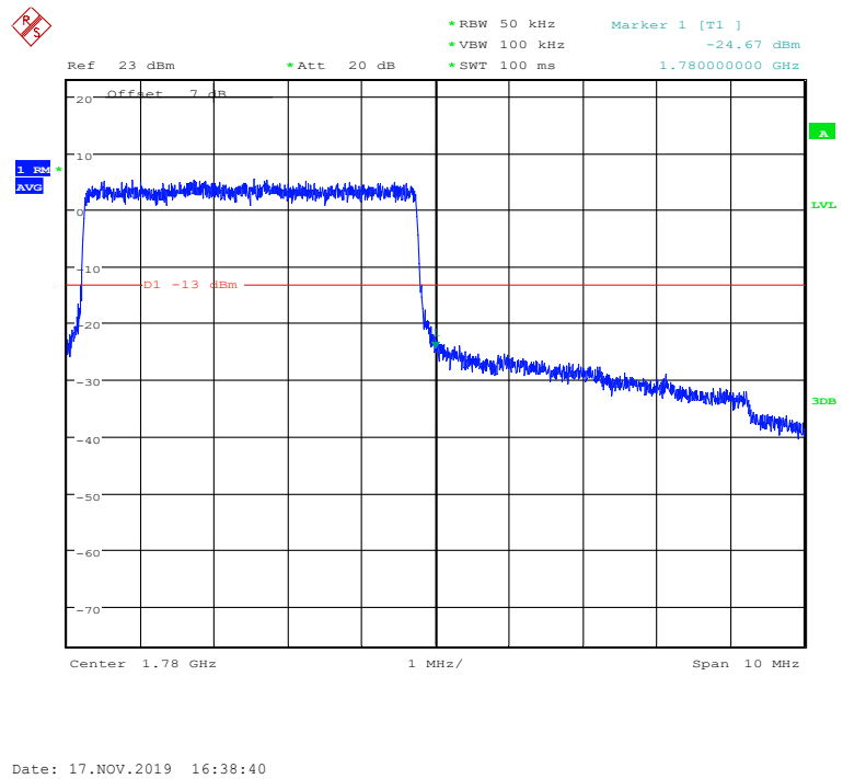
LTE Band66, 5MHz bandwidth, QPSK,(25,0) Mode, Above 1780MHz
