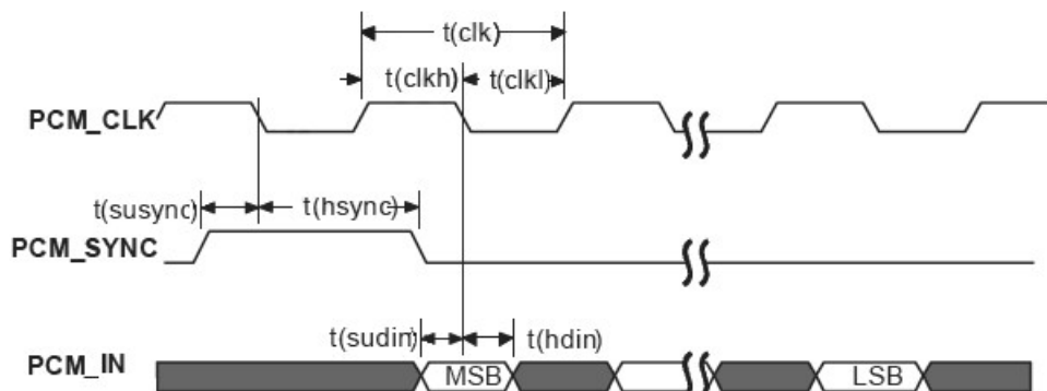
Figure 225: PCM_SYNC timing
