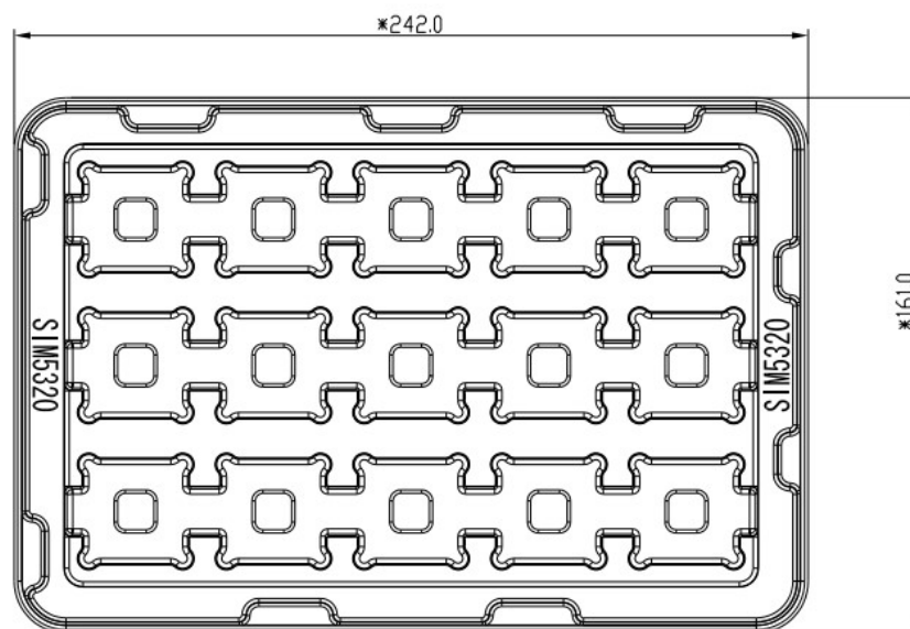
Figure 304: Tray drawing
