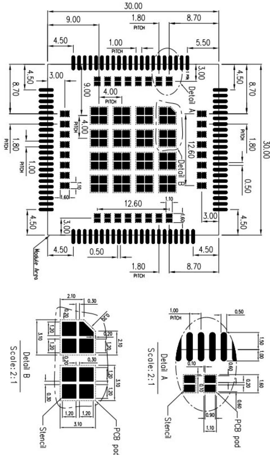
Figure 42 : Stencil Foil
