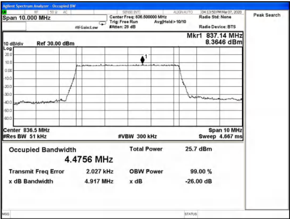
LTE Band26 QPSK 99% Channel 26915 BW=5MHz RB=25 RB Offset=0
