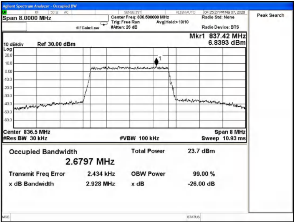
LTE Band26 16QAM 99% Channel 26915 BW=3MHz RB=15 RB Offset=0
